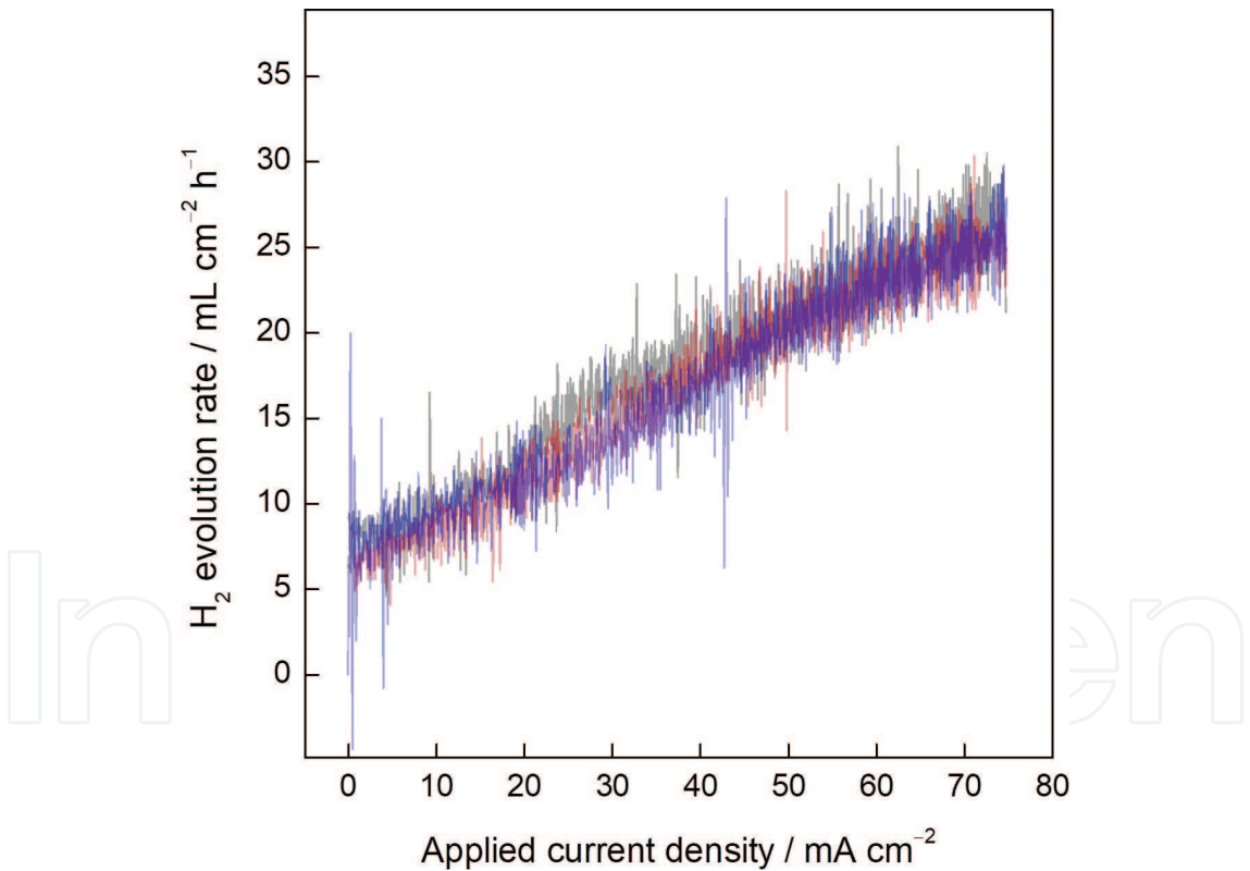
Figure 7. H 2 evolution rates for a high purity Mg electrode in 0.1 M citric acid buffer (pH 3) solution during anodic GDP as a function of the applied current density [16].
