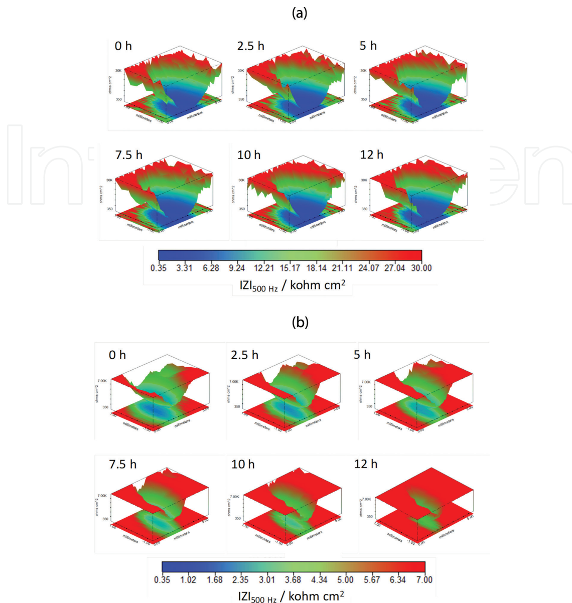
Figure 13. Impedance maps recorded at constant frequency (500 Hz) and variable soaking time in 0.006 M NaCl solution for (a) undoped sol-gel film and (b) 0.3% wt.% BTA doped sol-gel film deposited on AZ31 alloy.
