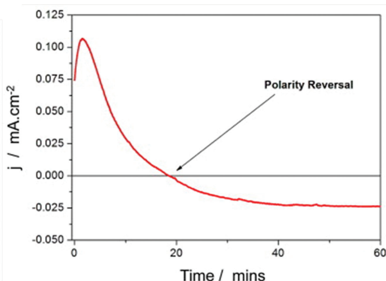
Figure 5. Net current density measured during PSP of high purity Mg at -1.6 V_{\text{SCE}} in NaCl solution [13].
