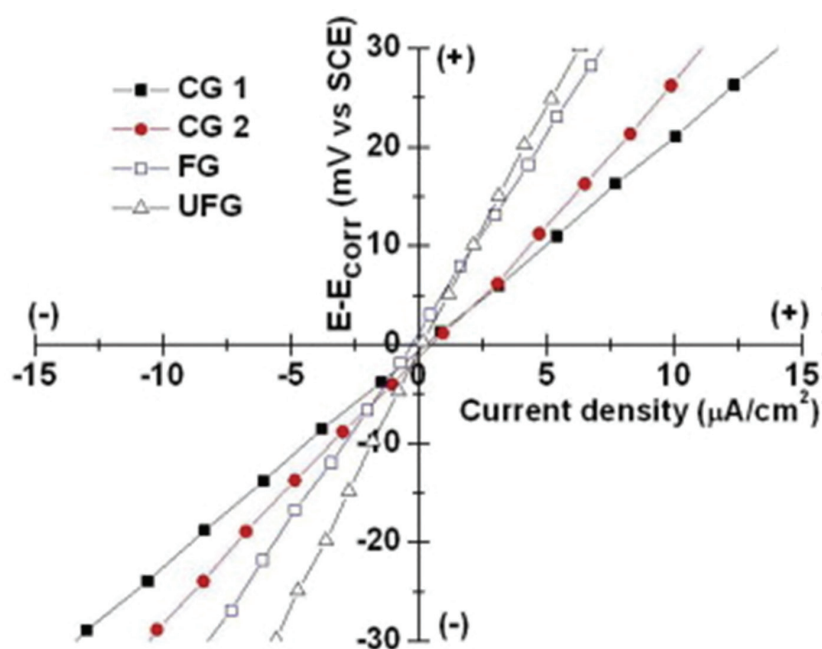
Figure 4. Linear polarization resistance plots of different conditions of Mg-Y-RE alloy in 3.5 wt.% NaCl [11].
