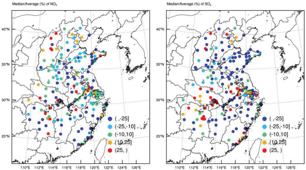
Figure 3. The distribution of the ratio of forecast bias median to the observational average in December, 2015 for \text{NO}_2 (left) and \text{SO}_2 (right).
