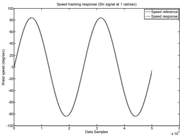
Fig. 9. With a 1 rad/s sinusoidal reference and a 1kg load over the joint.
