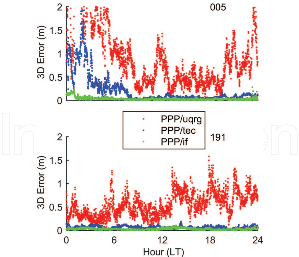
Figure 3. 3D error of PPP at ONRJ station on 2013 for DOY 005 during summer (top panel) and DOY 191 during winter (bottom panel).
