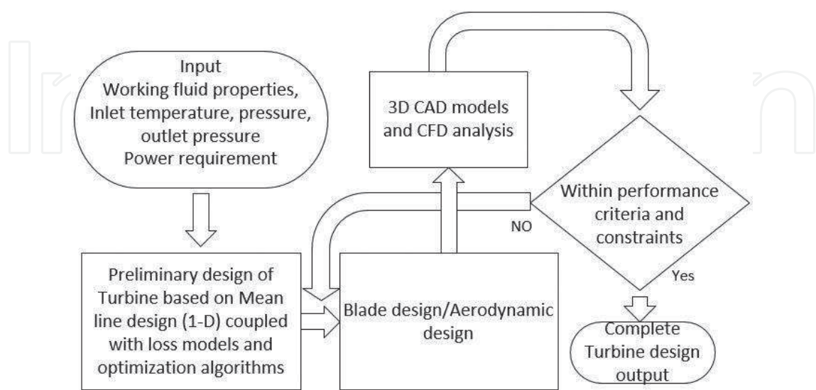
Figure 4. The fluid dynamic design process of turbine design.
