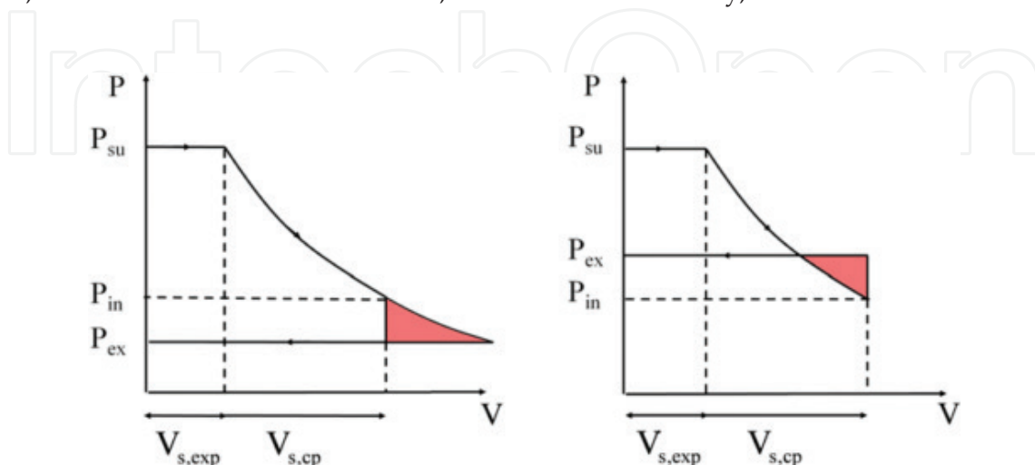
Figure 6. The under expansion (left) and over expansion (right) losses.
