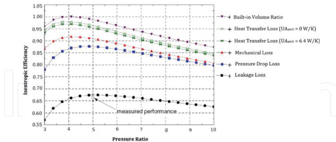
Figure 8. Variation in efficiency as a function of pressure ratio.
