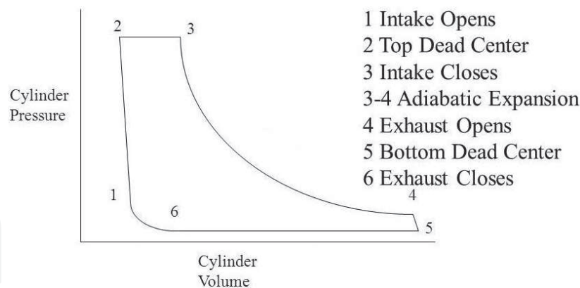
Figure 11. Pressure-volume diagram of piston expander.
