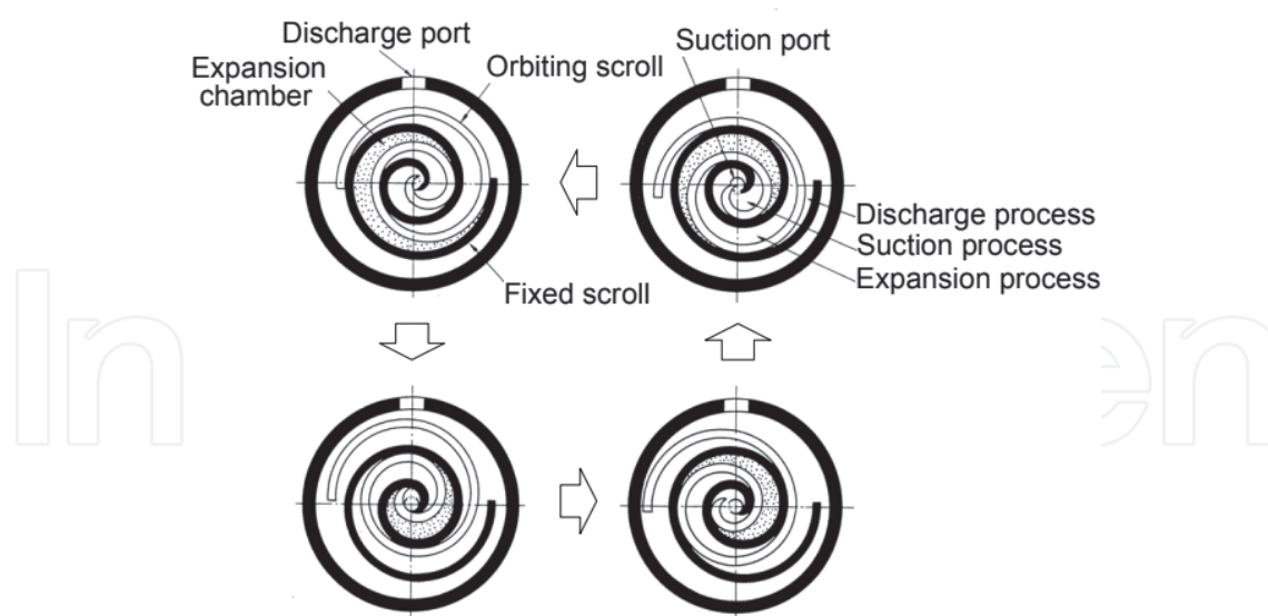
Figure 7. Operation of the scroll expander.
