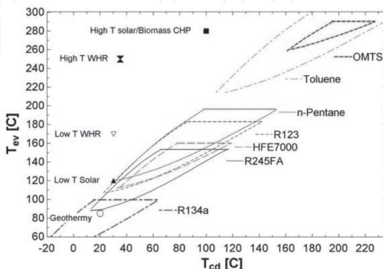
Figure 10. Selection maps for screw expander application.
