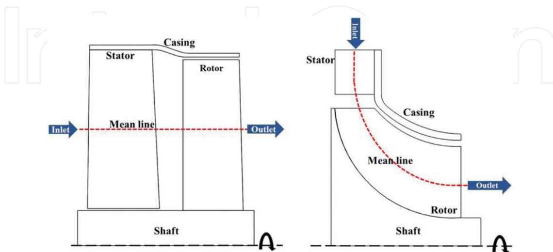
Figure 1. Schematic of axial flow (left) and radial inflow (right) turbines.
