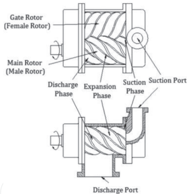
Figure 9. Schematic of a twin screw expander.
