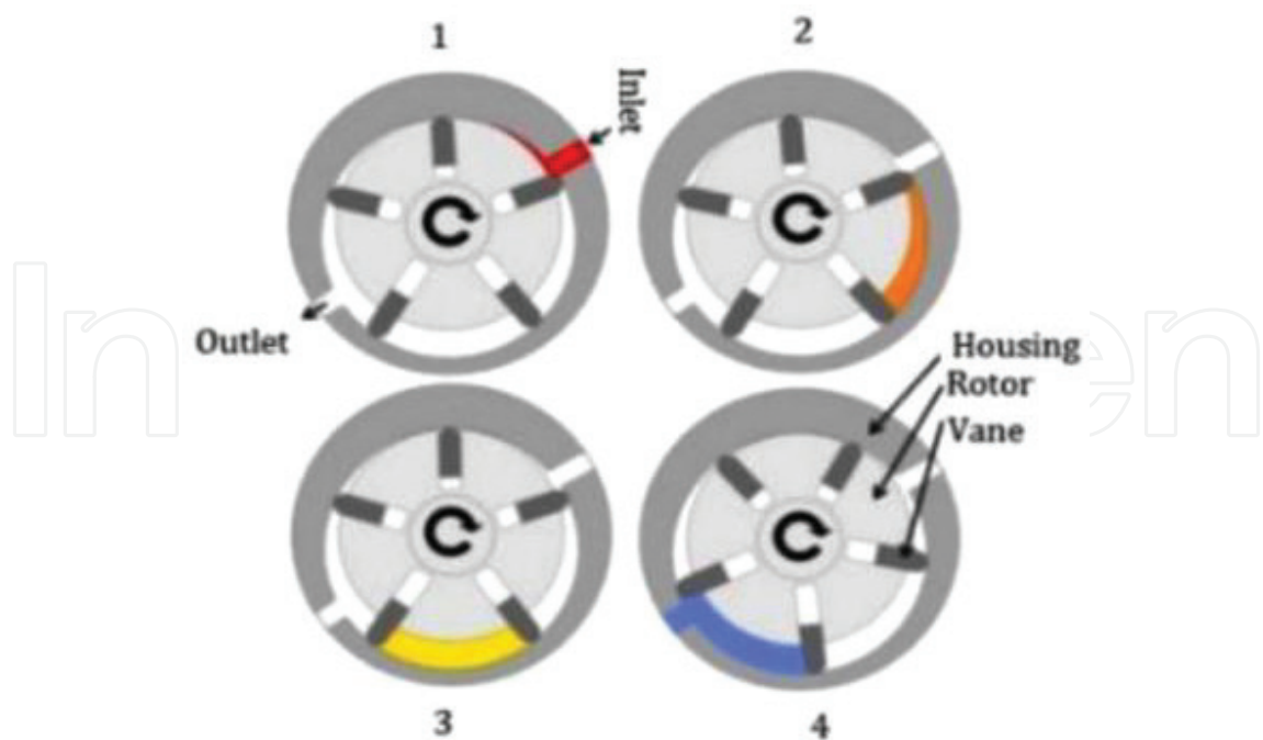
Figure 12. Operation of a rotary vane expander.
