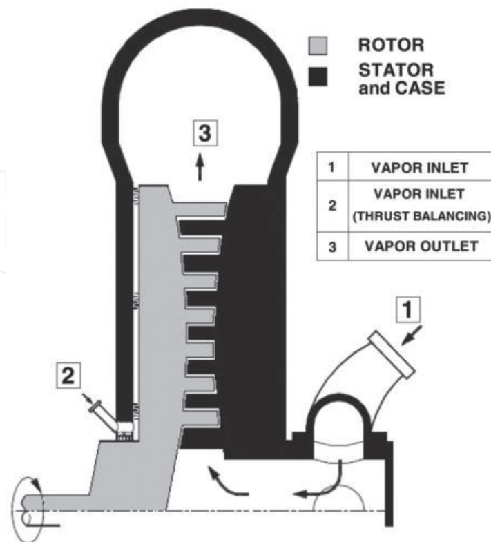
Figure 5. Schematic of radial outflow turbine.
