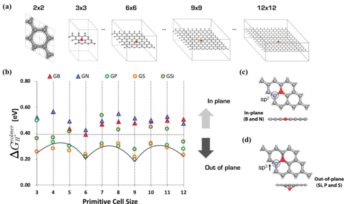
Figure 3. (a) Primitive cells of single heteroatom doped-graphene (GX, where G means graphene and X is B, N, Si, P, and S dopant) and (b) HER activities \Delta G_{H^+}^{Volmer} of GX as a function of primitive cell size. Red mark indicates dopant. There are two different types of structures depending on dopant, (c) in-plane and (d) out-of-plane.
