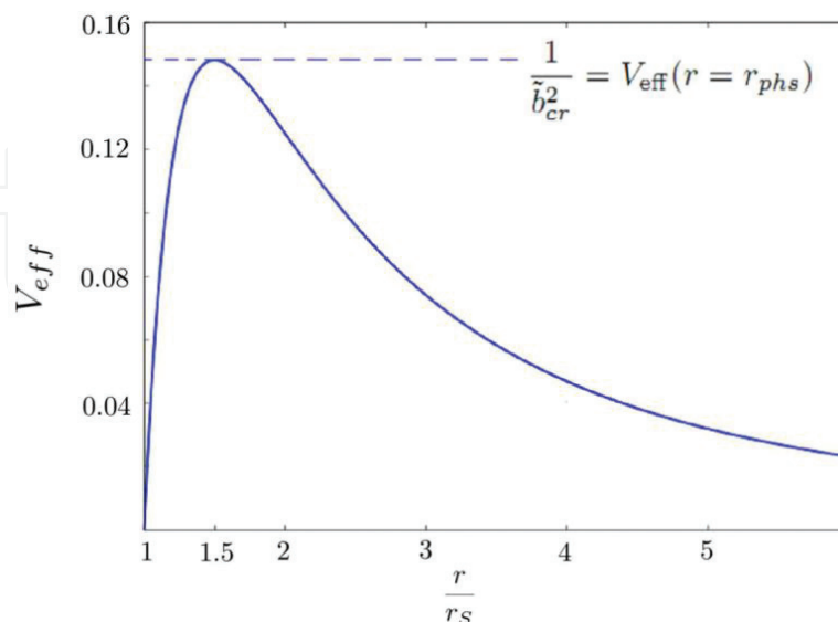
Figure 1. Effective potential V_{\text{eff}}(r) = f \frac{r_g^2}{r^2} in the case of Schwarzschild spacetime (horizontal axis— r expressed in units, r_S \equiv r_g = 2M ).
