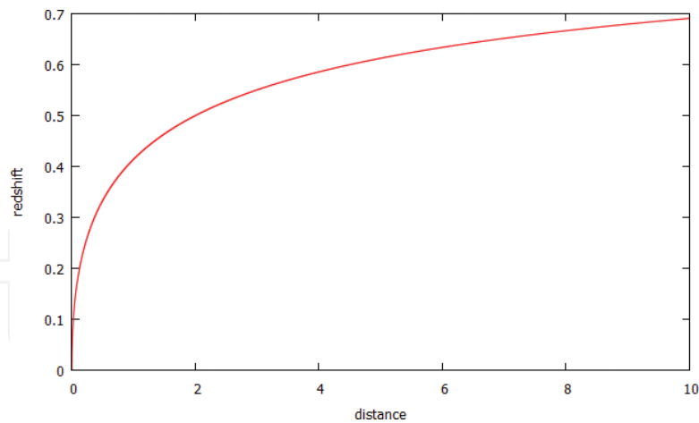
Figure 3. Monotonic and continuous change of the frequency ratio \frac{\omega^r}{\omega_{MS}^r} (redshift—Vertical axis) outside and inside the horizon (horizontal axis— r expressed in units M , r_g = 2 ).
