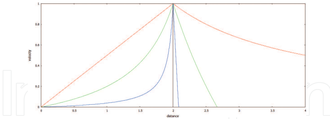
Figure 2. Values of ‘velocity’ V^2 measured by SO (outside horizon) and \tilde{V}^2 by RO (inside horizon) of different test particles in the Schwarzschild spacetime. The red curve corresponds to e = 1 , \tilde{V}^2 = \frac{r}{r_g} , the green curve to e = 0.5 and the blue one to e = 0.2 . The vertical line represents the horizon located at r_g = 2 (horizontal axis— r expressed in units M ).
