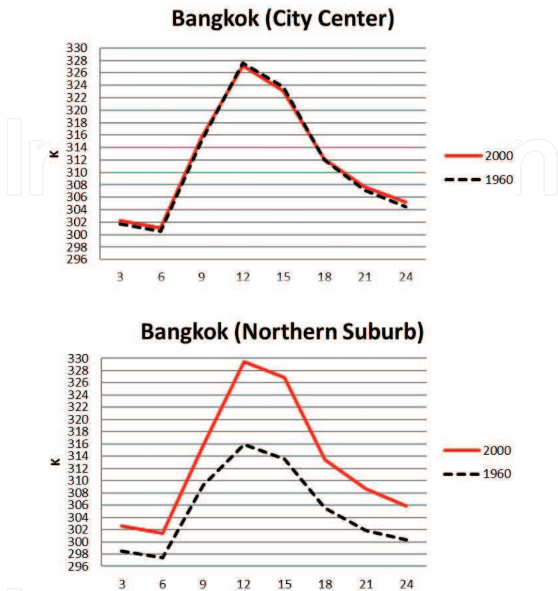
Figure 14. Diurnal variability of computed T_{sfc} in the hottest season (calm and clear day) in two stages [28]. Difference of computed warming of T_{sfc} in the same term (Bangkok).
