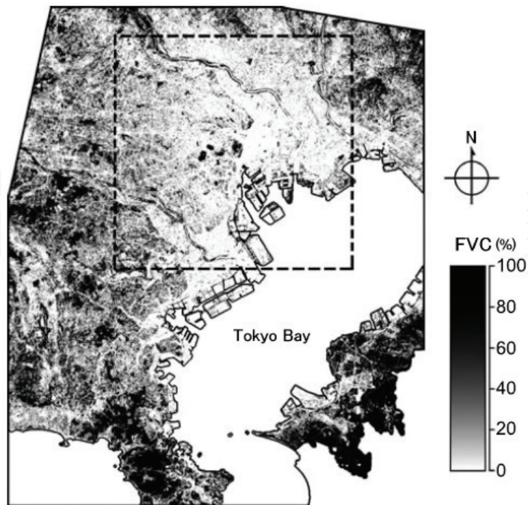
Figure 9. Estimated FVC (Fractional Vegetation Cover) around Tokyo [17]. The dashed-square indicates the target area of Figure 10.
