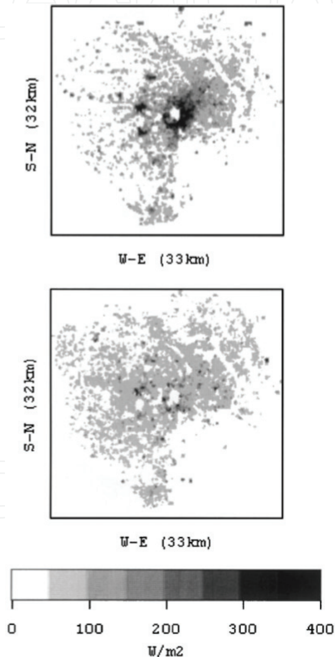
Figure 7. Distribution of anthropogenic heat in Tokyo at 2 p.m. (upper) and 9 p.m. (lower) in winter [12].
