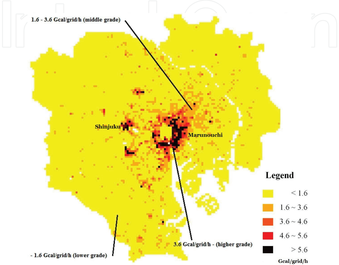
Figure 3. Distribution of heat demand density in Tokyo (daytime, winter, grid size: 250 m) [4].
