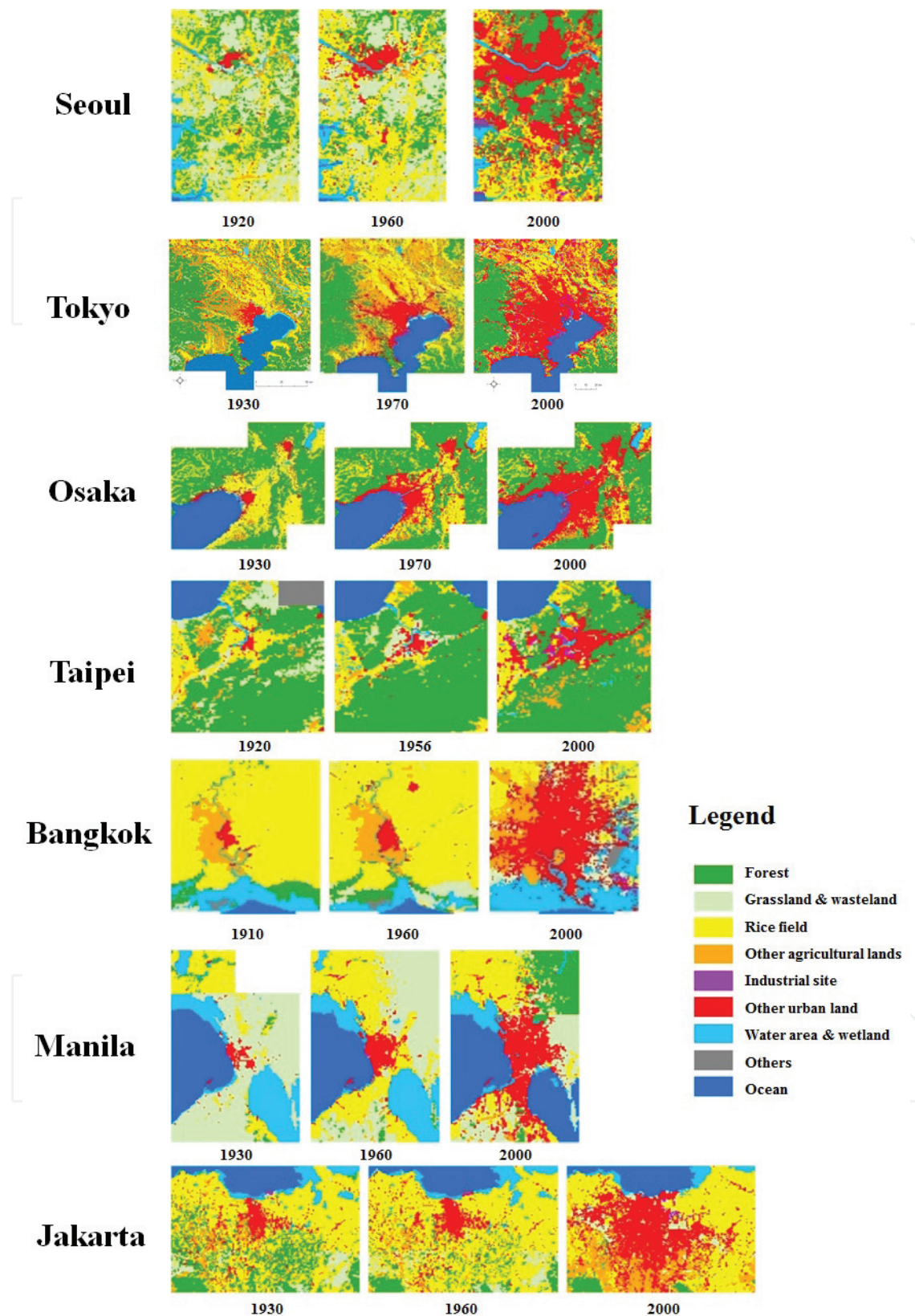
Figure 11. Urbanization around seven megacities in Asia (RIHN Research Project C-5 “Human Impacts on Urban Subsurface Environments”) [28].
