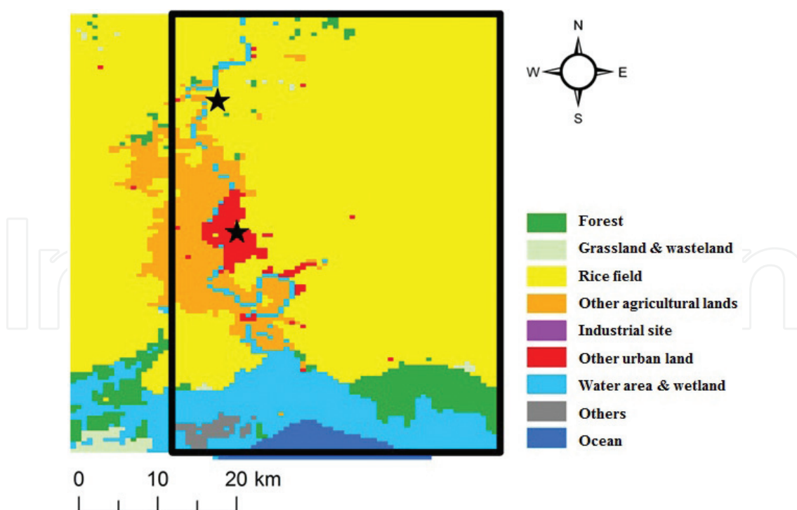
Figure 12. Land-cover/use around Bangkok in 1910 with its legend [28]. Stars show “City Center” and “Northern Suburb”. Inside of solid rectangle line shows the areas displaying computed results in Figure 13 .
