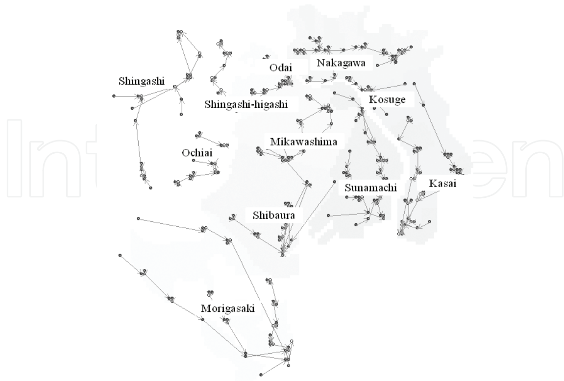
Figure 2. Extracted sewerage lines and sewerage treatment districts in the 23 special wards of Tokyo Metropolis [4]. (N-S: 32 km, E-W: 33 km).
