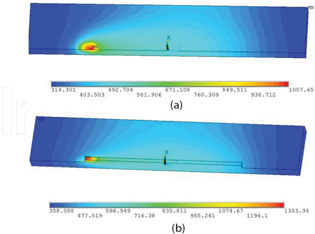
Figure 18. Temperature distribution, K (a) t = 291 s, (b) t = 506 s.
