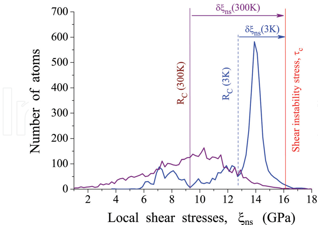
Figure 6. Distributions of local shear stresses \xi_{ns} (in the slip system ([1\bar{1}\bar{1}](211)) for instability point R_C in Fe-nanowire under uniaxial tension in [100] direction at T = 3 K and T = 300 K [37].
