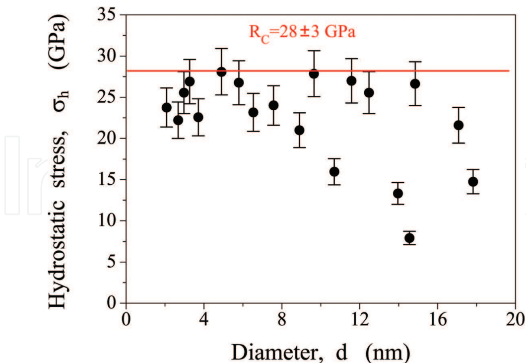
Figure 11. Hydrostatic tensile strength of tungsten nanocrystals at 77 K; d is the diameter of nanocrystal region fractured under hydrostatic tension; R_C is the experimental evidence of strength.
