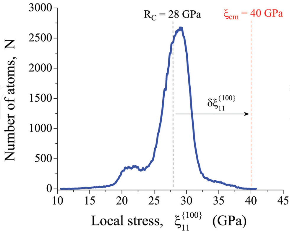
Figure 10. Distribution of local normal stresses \xi_{11}^{\{100\}} in the ball-shaped nanosized specimen at the moment of its instability at T = 77 K: R_C is the global stress of instability of the ball-shaped nanosized specimen; \xi_{cm} is local critical stress of bcc \rightarrow fcc transition; \delta\xi_{11}^{\{100\}} is local stress fluctuation on {100} planes, required for realisation of the local instability of crystal.
