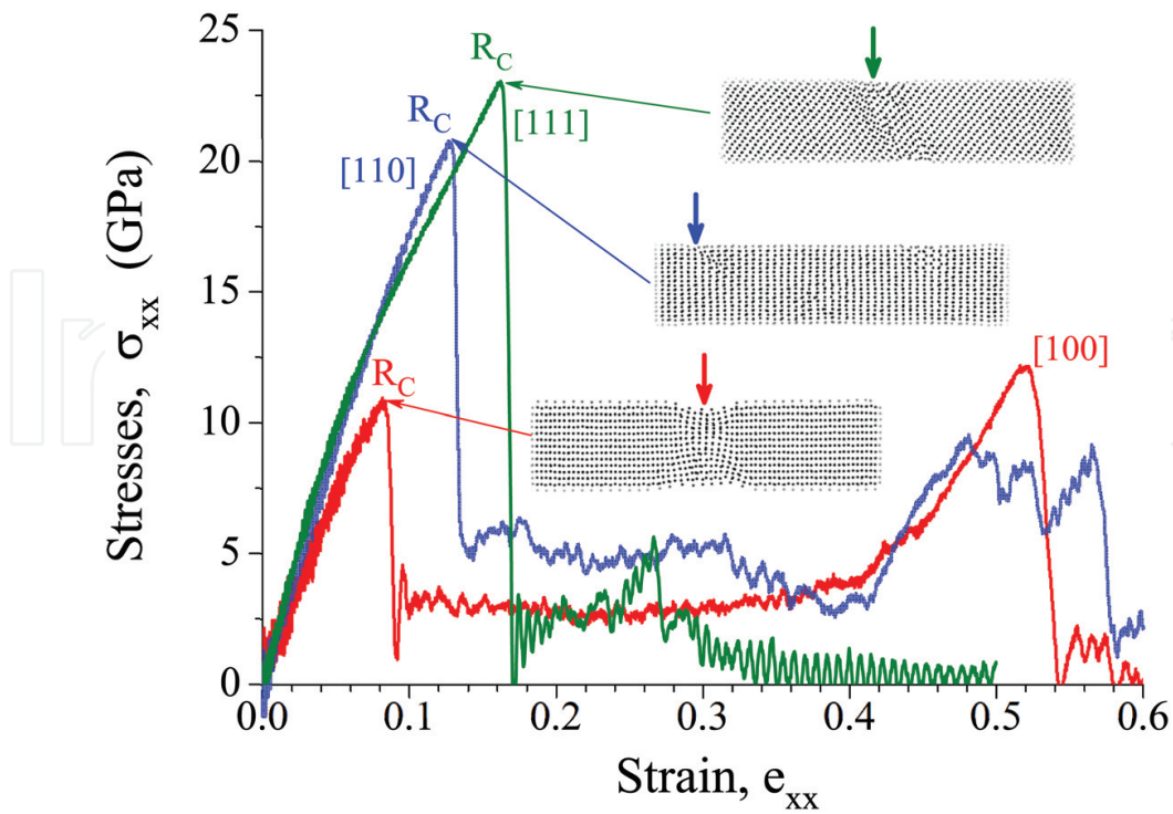
Figure 3. Images of Fe-nanowires and diagrams of their strain at temperature 300K for three crystallographic orientations: arrows indicate instability regions; R_C is the instability stress (strength of nanowire).
