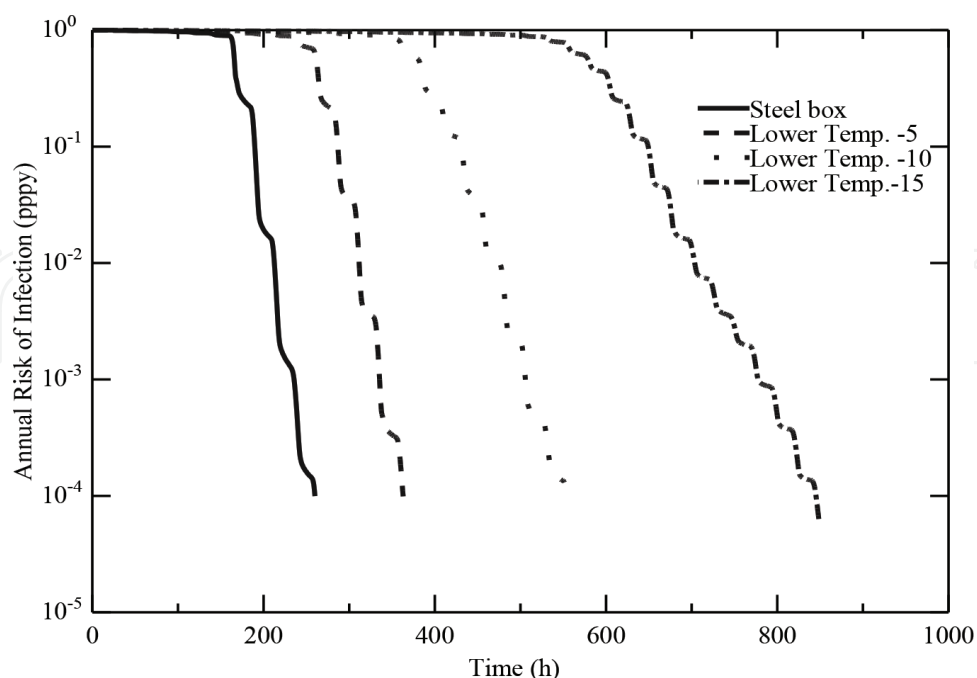
Figure 8. Norovirus annual infection risk with post-treatment.
