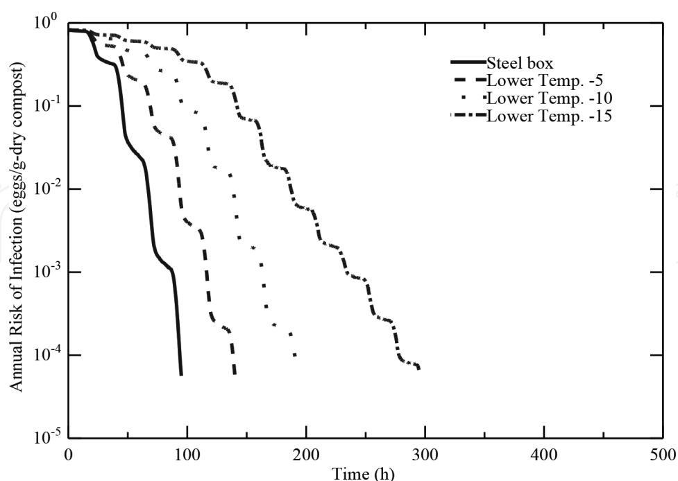
Figure 7. Ascaris annual infection risk associated with post-treatment.
