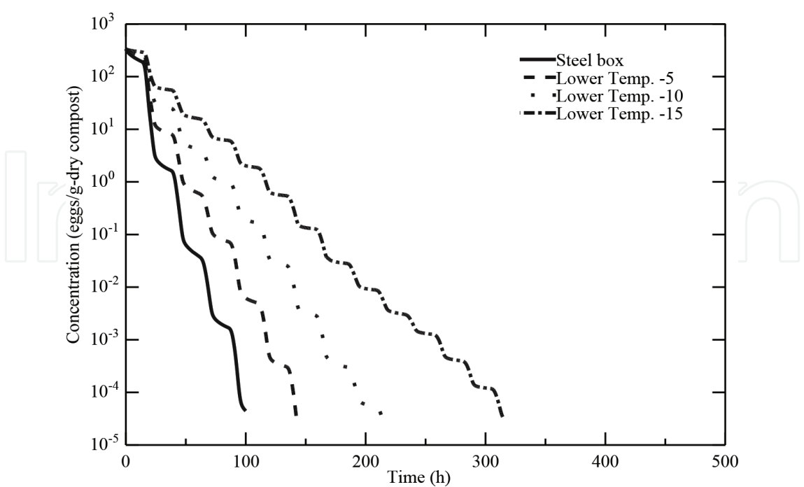
Figure 4. Change in Ascaris eggs concentration for the post-treatment.
