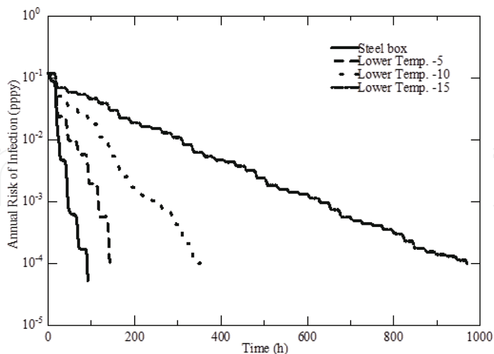
Figure 9. Salmonella annual infection risk associated with post-treatment.
