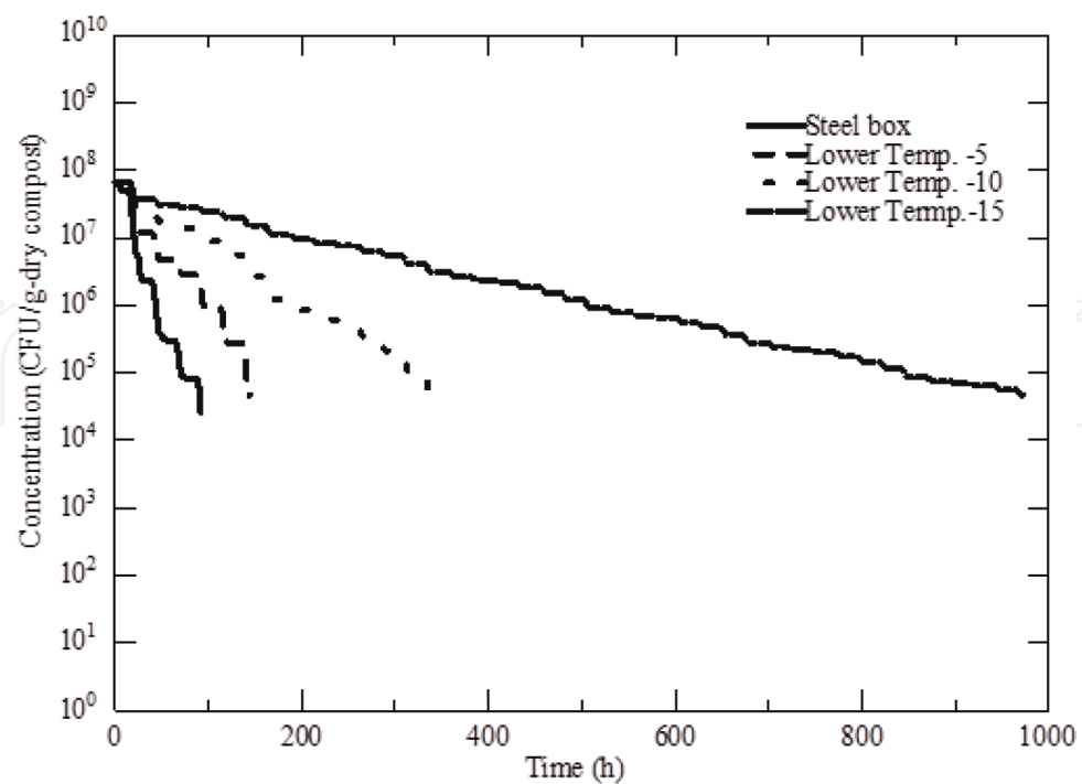
Figure 6. Change in Salmonella concentration.
