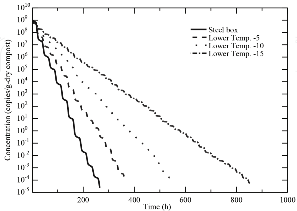
Figure 5. Change in norovirus concentration for post-treatment.
