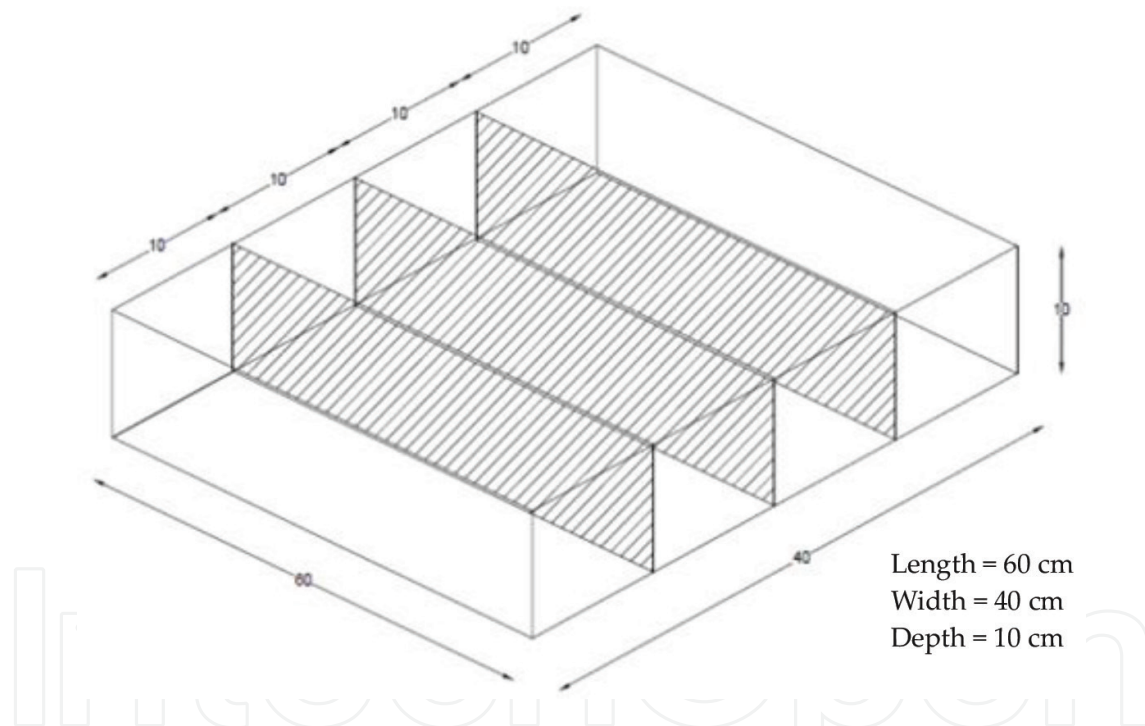
Figure 2. A proposed compost solar sanitisation installation that could reduce the heat loss [4].
