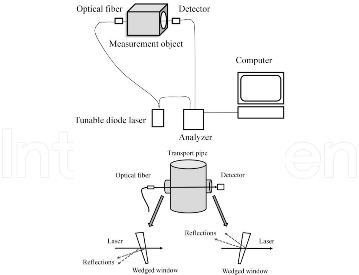
Figure 6. Typical geometric arrangement of TDLAS. (a) Typical geometric arrangement. (b) Wedged windows used in the laser pass.
