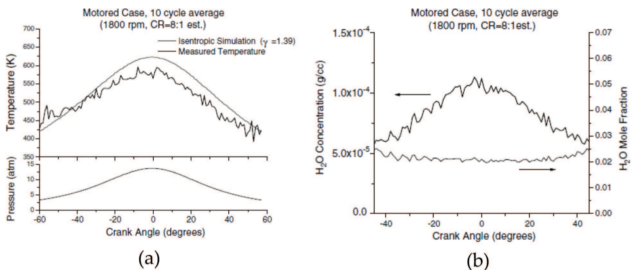
Figure 9. Gas temperature and \text{H}_2\text{O} concentration measurement in a motoring, single-cylinder engine. (a) Measured temperature. (b) Measured \text{H}_2\text{O} concentration [26].
