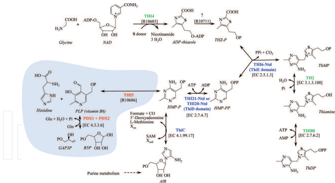
Figure 3. Thiamin (vitamin B1) biosynthesis in eukaryotes. Blue shading indicates restricted to yeast. Abbreviations: ADP-thiazole, ADP-5-ethyl-4methylthiazole-2-carboxylate; PLP, pyridoxal phosphate; R5P, D-ribose 5-phosphate.?, not determined to date. For additional abbreviations and coloring scheme see Figure 2 .
