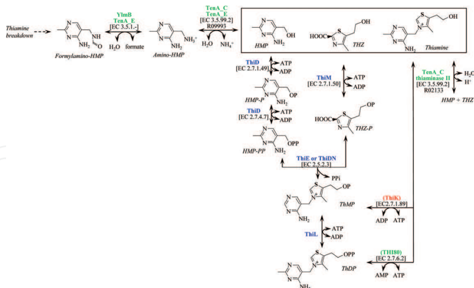
Figure 6. Thiamin (vitamin B1) salvage in archaea. Abbreviations: Formylaminio-HMP, N-formyl-4-amino-5-aminomethyl-2-methylpyrimidine; amino-HMP, 4-amino-5-aminomethyl-2-methylpyrimidine; HMP, 4-amino-5-hydroxymethyl-2-methylpyrimidine; THZ, 4-methyl-5-(2-hydroxyethyl)thiazole. For additional abbreviations and coloring scheme see Figures 2-4 .
