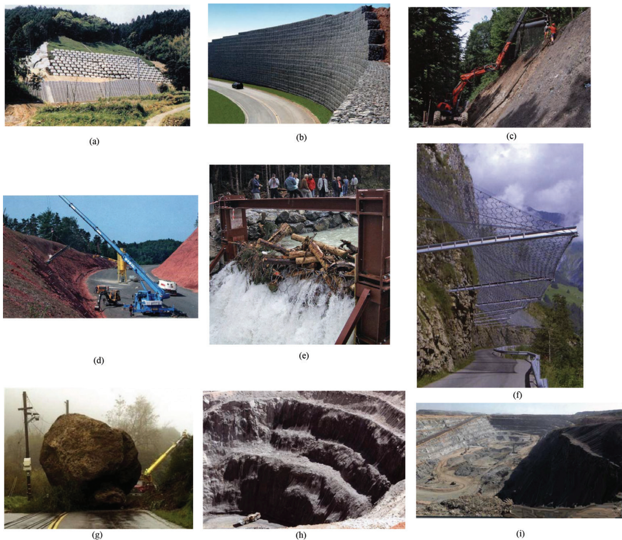
Figure 6. (a) Anchor construction—Japan. (b) Strengthen wall—Switzerland. (c) Slope defense by flexible metallic net—Switzerland. (d). Slope protection by flexible metallic net—Switzerland. (e). Barrier for retaining debris flow—Switzerland. (f) Ring metallic net protection above road against rockfall—Switzerland. (g) Big stone on the road. It is possible to make it fall down, to break, or to reinforce by cement on the slope of the road. (h) Rock slope surface stabilization and rockfall hazard mitigation using coated double-twist rockfall mesh. Australia. Mining company Barrick (Australia Pacific) Ltd., 2010. (i) Rockfall mitigation drapery using double-twist rockfall mesh—South Africa. Mining company Anglo-platinum, 2009.
