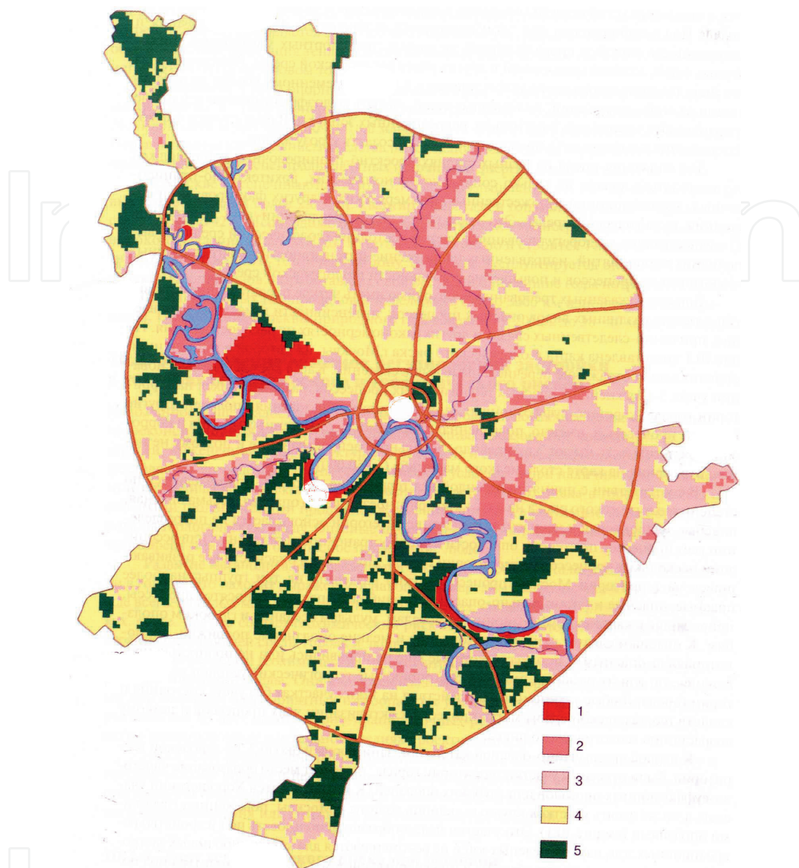
Figure 3. Map of geological danger in Moscow. Landslides, karst, and underflooding. (Osipov V.I., Kutepon V.M., Mironov O.K.) [1]. Landslides are near rivers in semi-dark (red and pink). 1: Very high danger, 2: High, 3: Middle, 4: Low, 5: No. white circles: Risk “hot spots.” Kremlin hill (center) and Vorobiovy Mountains (south-west).
