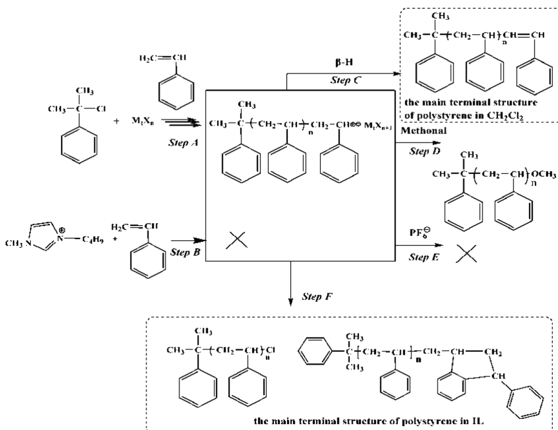
Figure 3. Polymerization pathway of cationic polymerization of styrene with CumCl/Lewis acid in [\text{bmim}][\text{PF}_6] .
