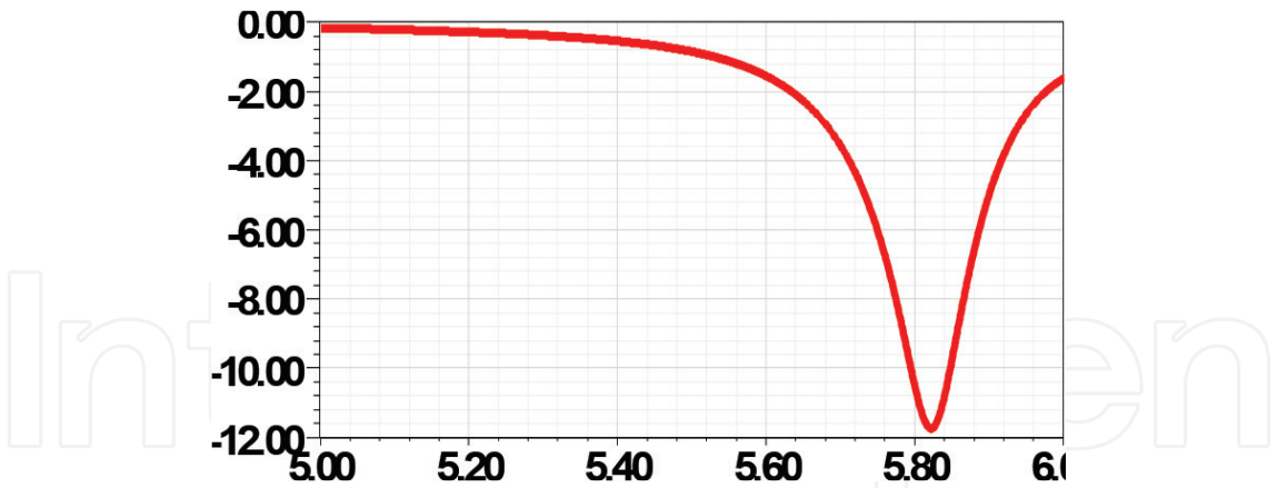
Figure 21. Return loss (Position 3).
