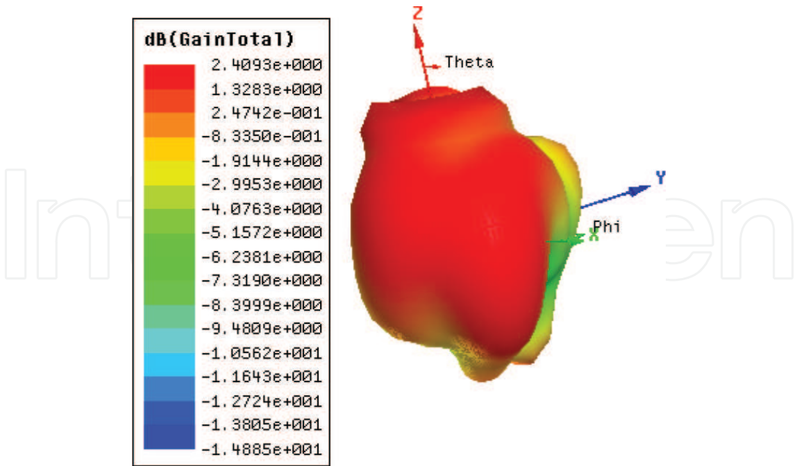
Figure 12. The 3D radiation pattern of the PIFA.
