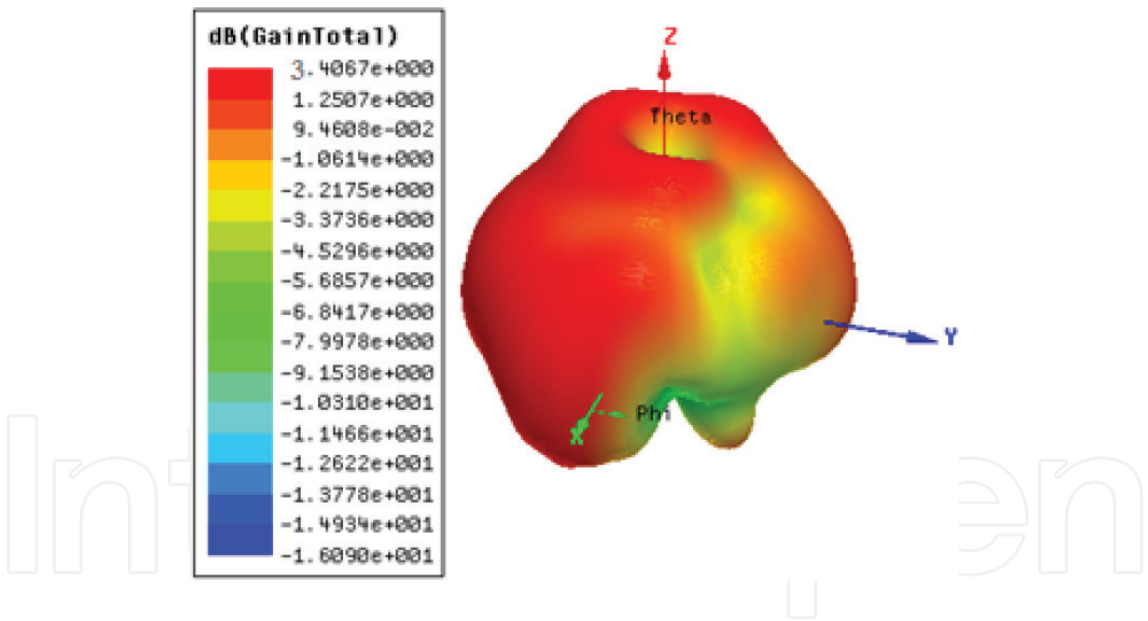
Figure 13. The 3D radiation pattern of the PIFA with T-slot.
