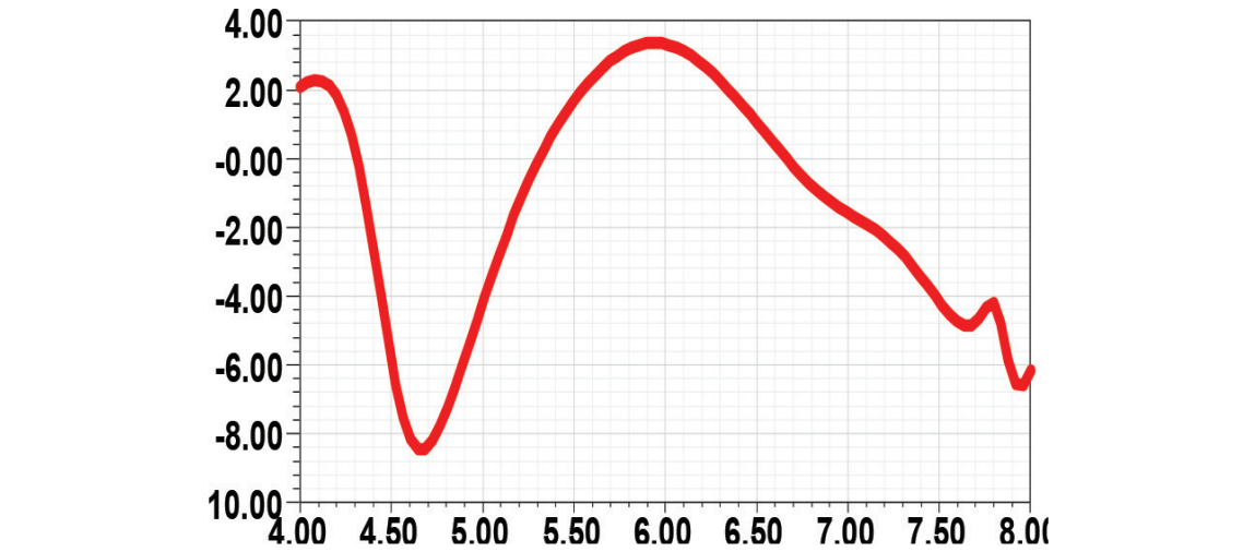
Figure 15. Gain of PIFA with slot.
