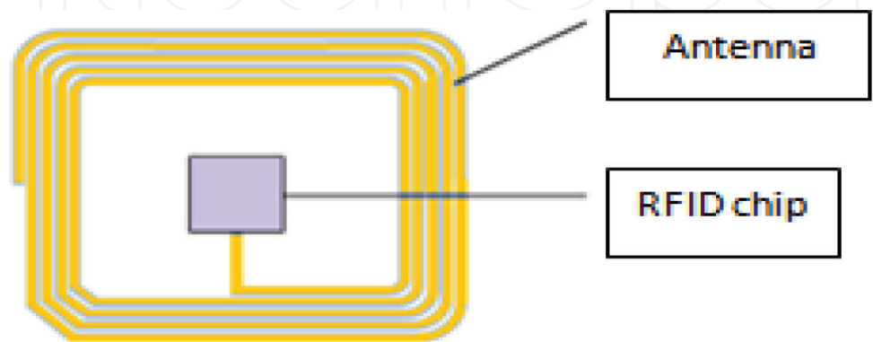
Figure 1. Tag antenna.
