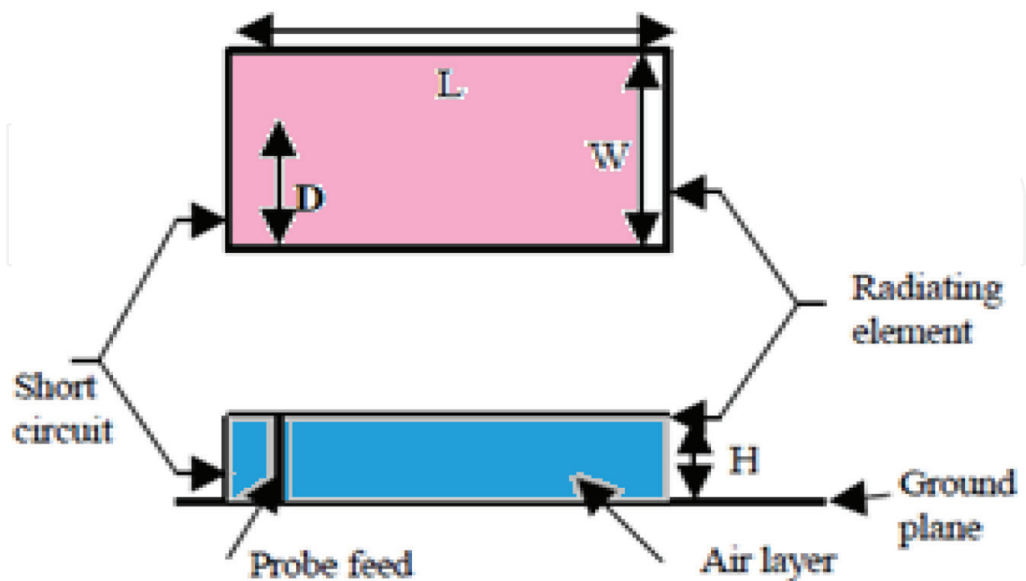
Figure 3. The PIFA.
