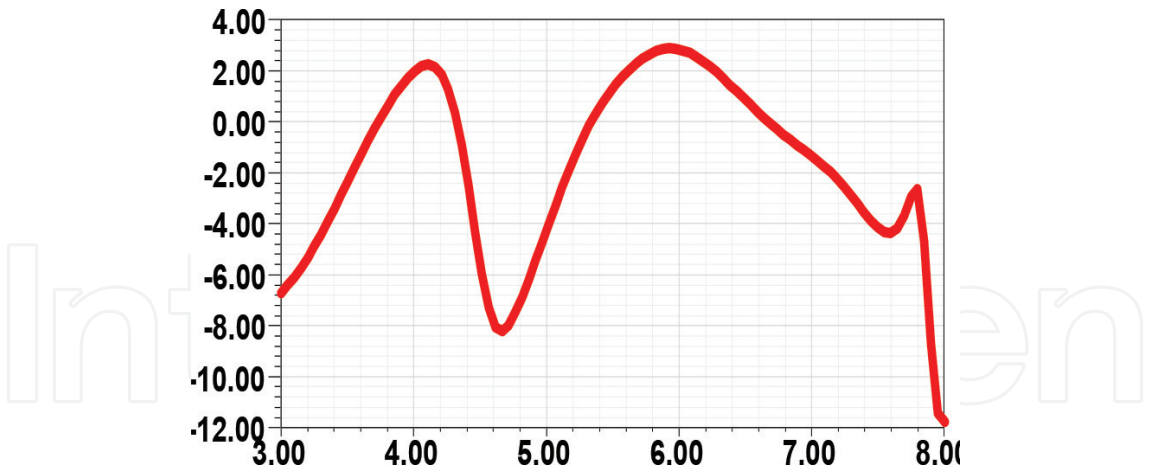
Figure 14. Gain of the PIFA.
