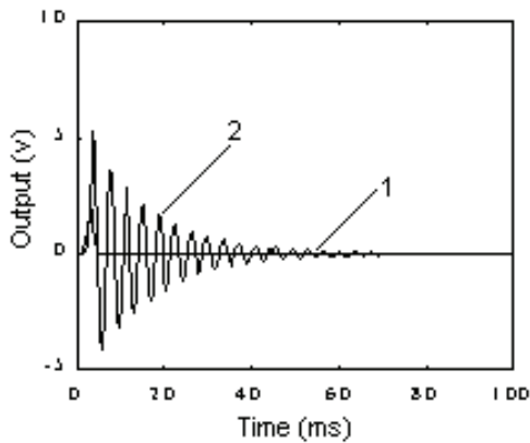
Fig. 6-5 Impulse input and nonlinear dynamic response: (1) impulse input, and (2) nonlinear dynamic response.
