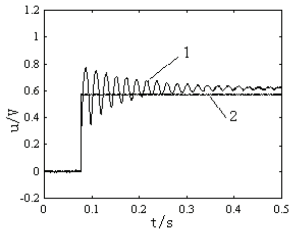
Fig. 6-29 Input and nonlinear output (1)nonlinear output, (2) input signal
