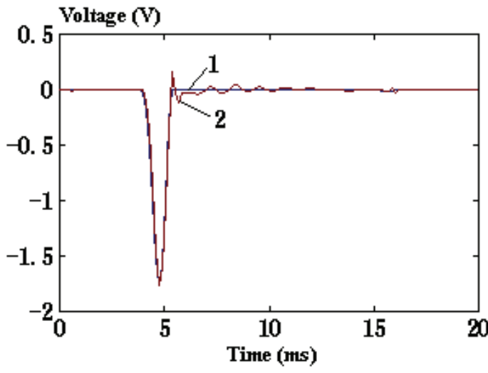
Fig. 5-4 (b) Decoupling and compensating result of direction Y
