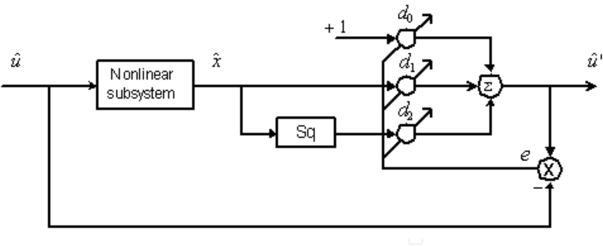
Fig. 6-12 A training schematic diagram of the FLANN
