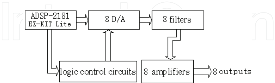
Fig. 6-26 Schematic block diagram of simulating system of sensors
