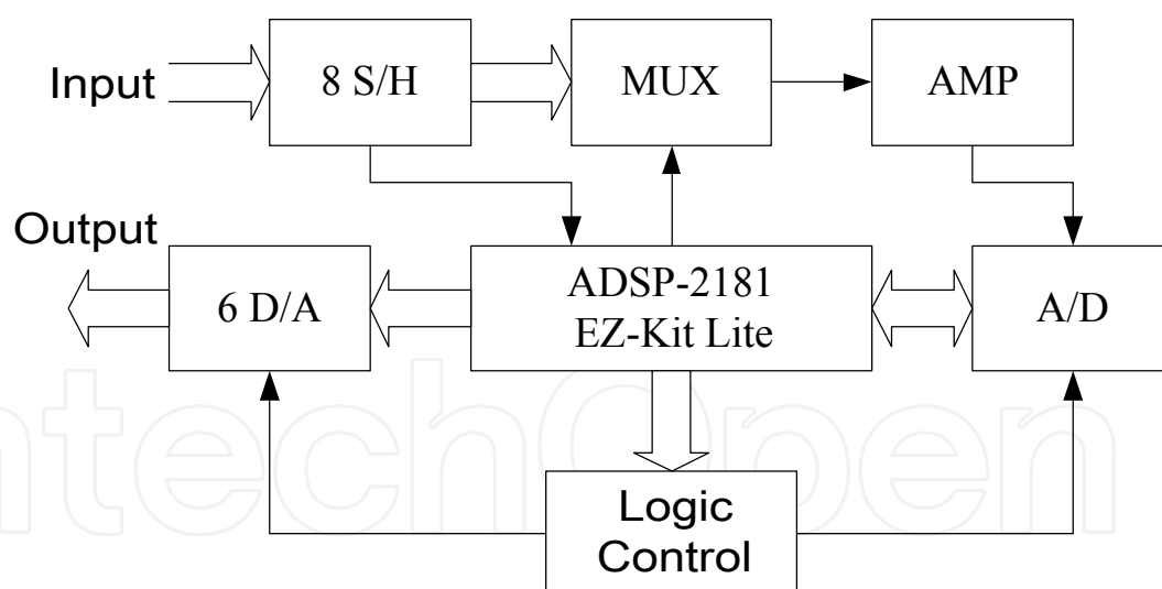
Fig. 4-2 Schematic block diagram of dynamic compensating system
