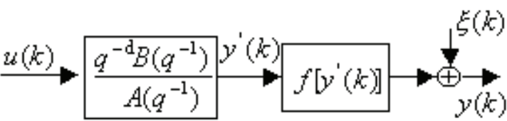
Fig. 6-21 Structure scheme of sensor after decomposition
