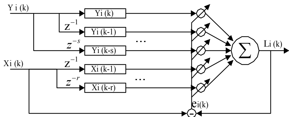
Fig. 5-2 Schematic of modeling by FLANN
