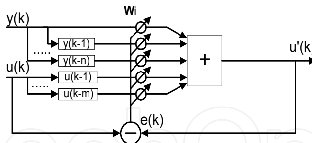
Fig. 4-1 Design schematic of dynamic compensating device by FLANN
