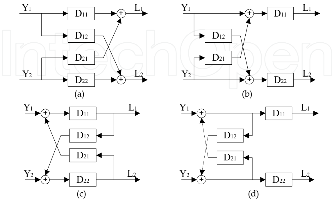
Fig. 5-1 Four kinds of network structures
