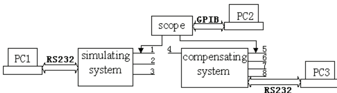
Fig. 6-28 Experimental setup
