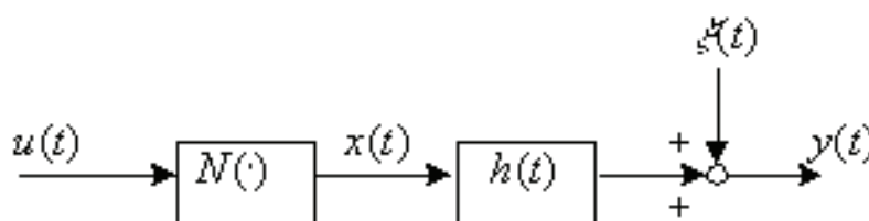
Fig. 6-1 Hammerstein model
