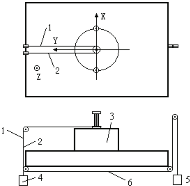
(b) Channel M_x
