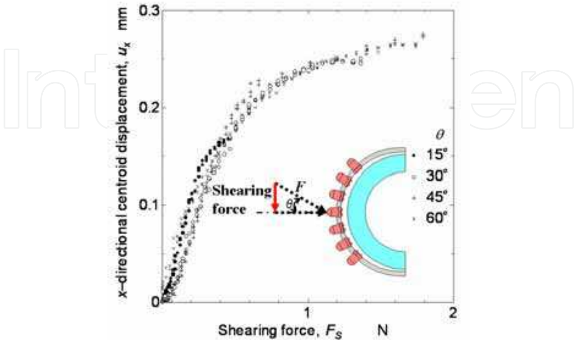
Fig. 11. Relationship between centroid displacement and applied shearing force
