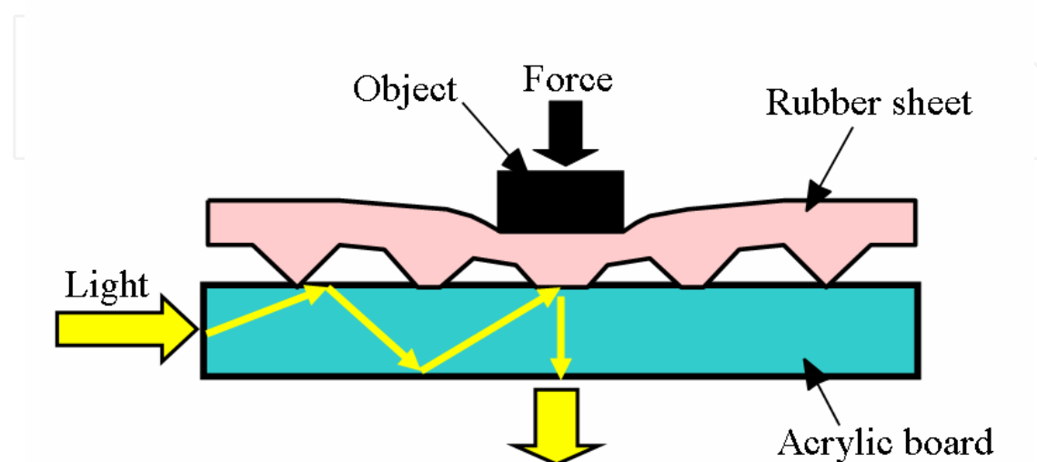
Fig. 1. Conventional optical tactile sensor
