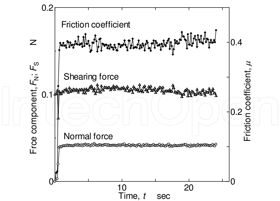
Fig. 17. Variation in force components and friction coefficient during scanning test (abrasive paper of 1 m and velocity of 6.2 mm/ sec)
