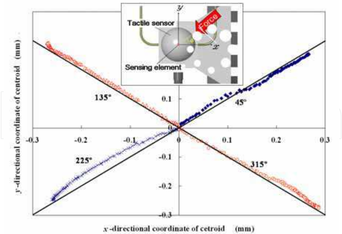
Fig. 12. Precision of two-dimensional shearing force detection
