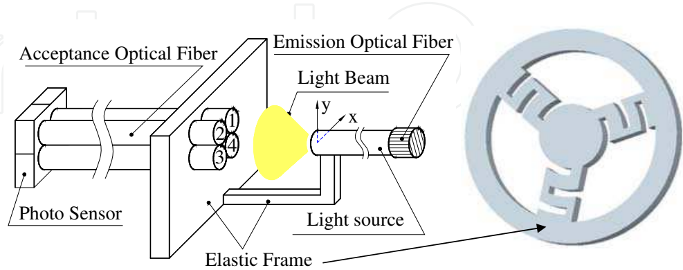
Fig. 3. Layout of the 6-axis optical force/torque sensor (Takahashi et al., 2003)
