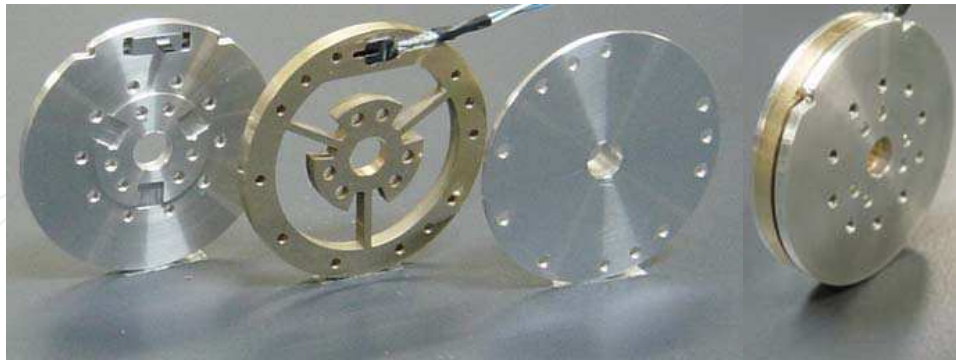
Fig. 9. Optical torque sensor with hub-spoke-shaped flexure
