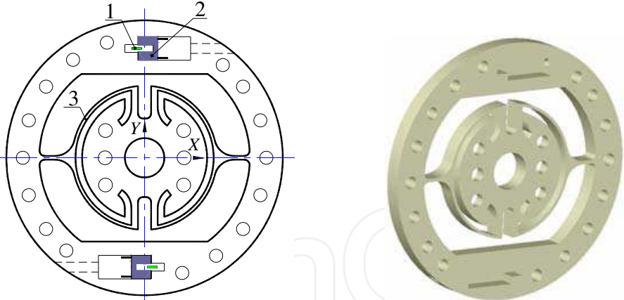
Fig. 13. Semi-ring-shaped spring
