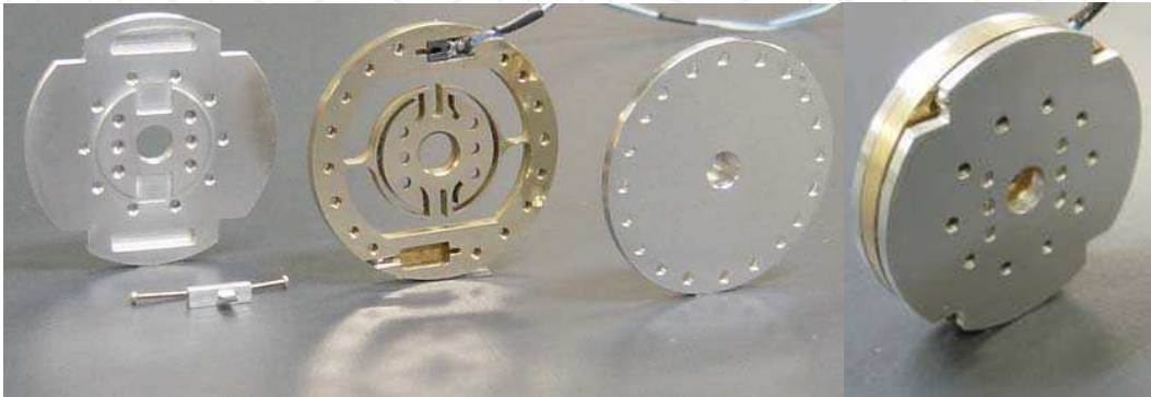
Fig. 15. Optical torque sensor with semi-ring-shaped flexure
