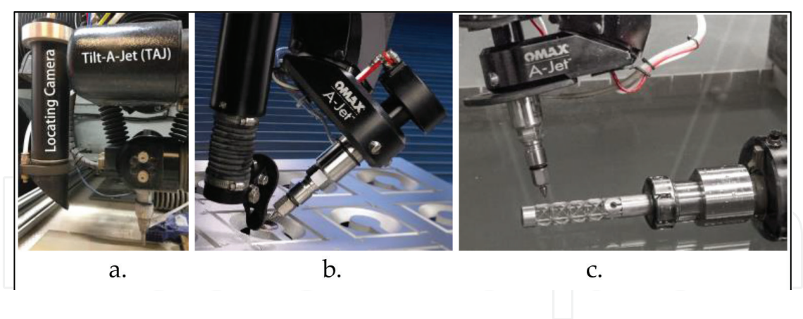
Figure 2. Accessories for 3D machining (a) TAJ (b) A-Jet (c) Rotary Axis.
