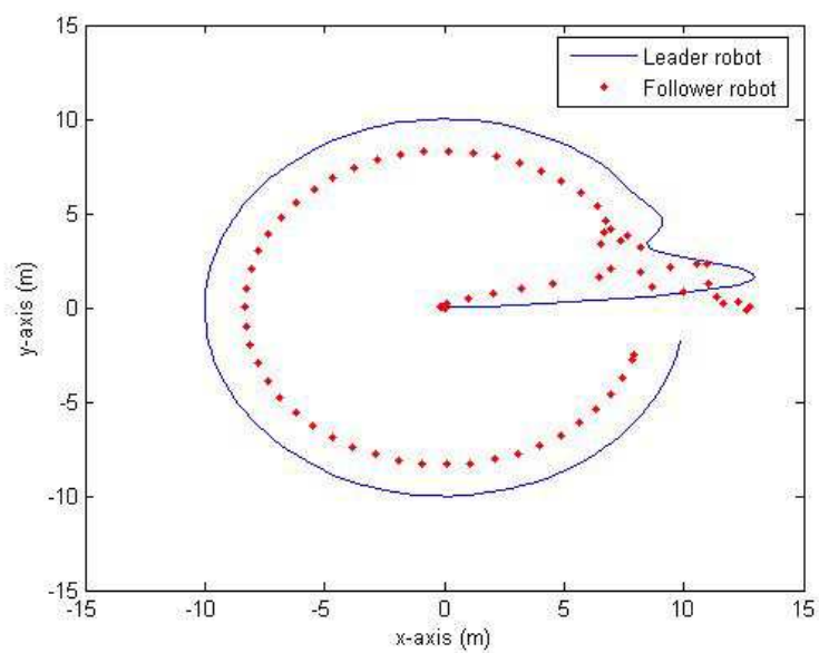
Fig. 10. Actual trajectory using separation bearing controller for Eq. (46) In another set of simulation, the separation bearing angle was changed as follows.
