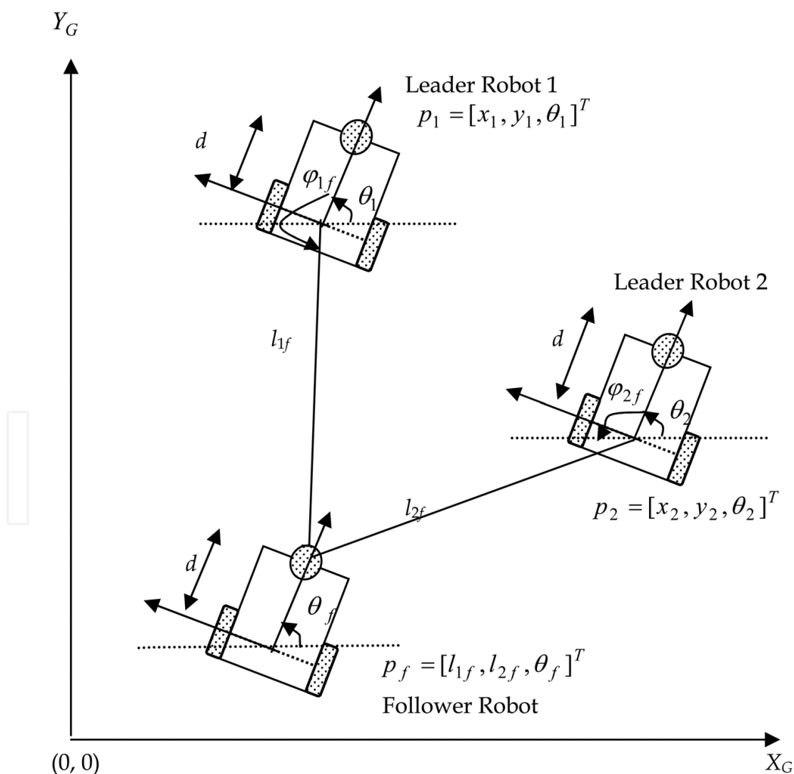
Fig. 2. Leader-follower formation using separation-separation controller.
