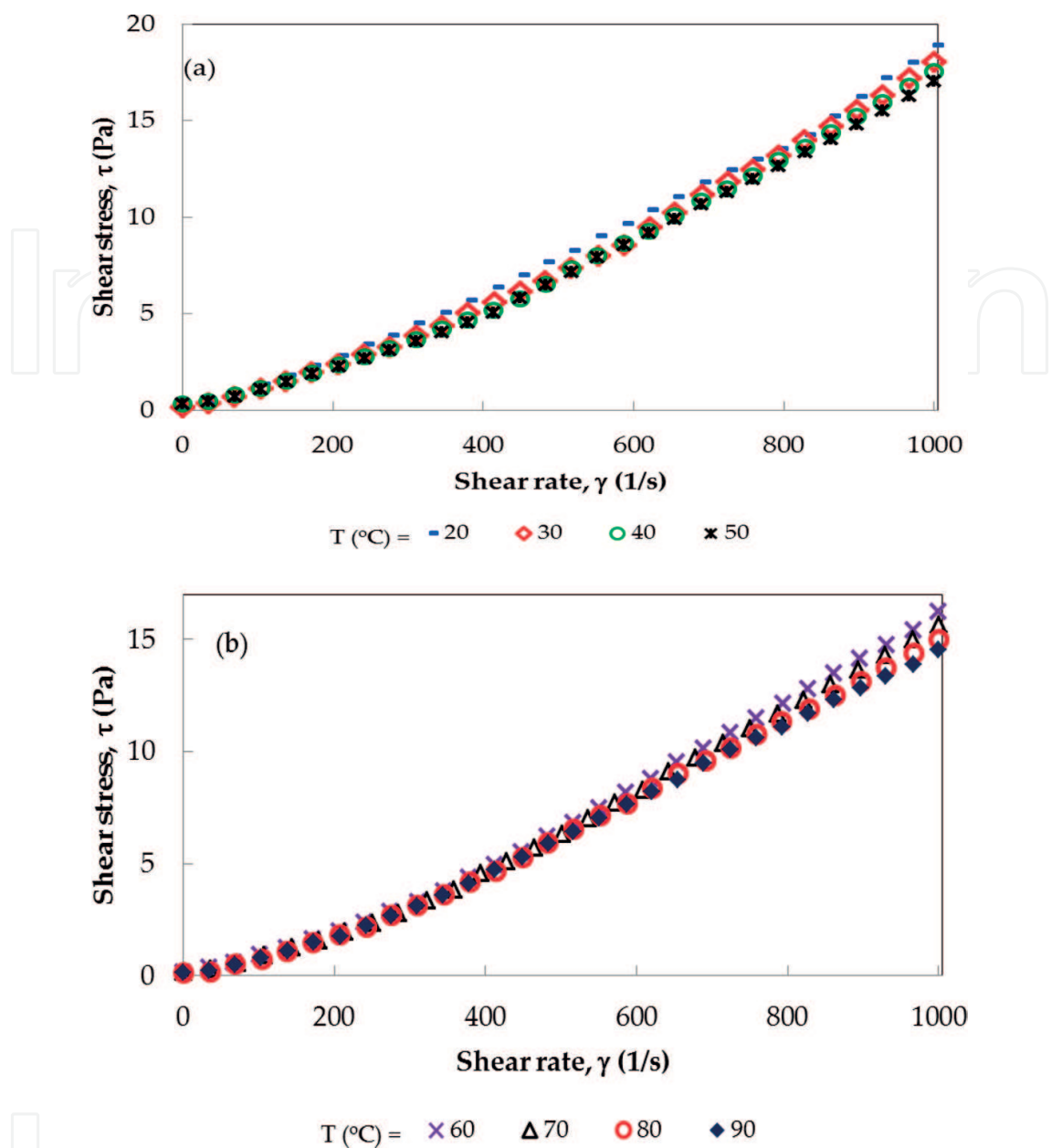
Figure 3. Rheogram behavior of crude oil emulsion at \phi = 0.20 . (a) Temperature (°C): \blacksquare = 20^\circ\text{C} , \color{red}\blacklozenge = 30^\circ\text{C} , \color{green}\bullet = 40^\circ\text{C} and \times = 50^\circ\text{C} . (b) Temperature (°C): \times = 60^\circ\text{C} , \blacktriangle = 70^\circ\text{C} , \color{red}\bullet = 80^\circ\text{C} and \color{blue}\blacklozenge = 90^\circ\text{C} .
