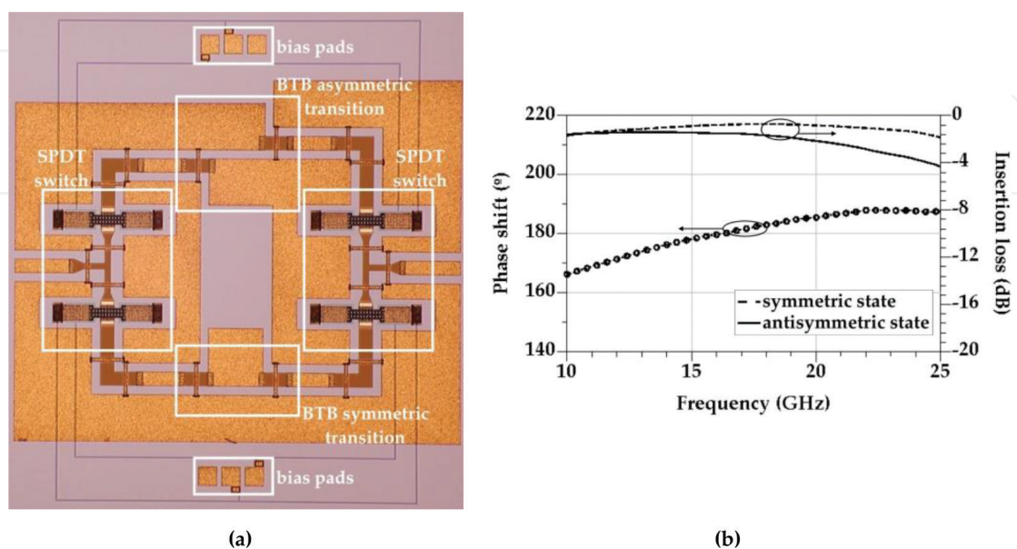
Figure 21. (a) Manufactured 180^\circ phase switch. (b) Measured insertion loss (symmetric and antisymmetric paths) and measured phase shift between the two paths.
