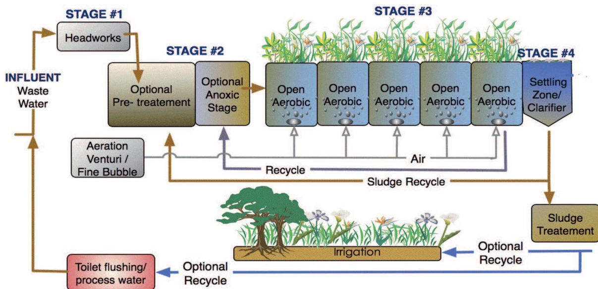
Figure1. Ecologicalsewagetreatment( http://ingenious.com/sectors/the-environment/eliminating-waste-and-inefficiency/sewage-treatment-via-bionutrient-recycling/ ).
