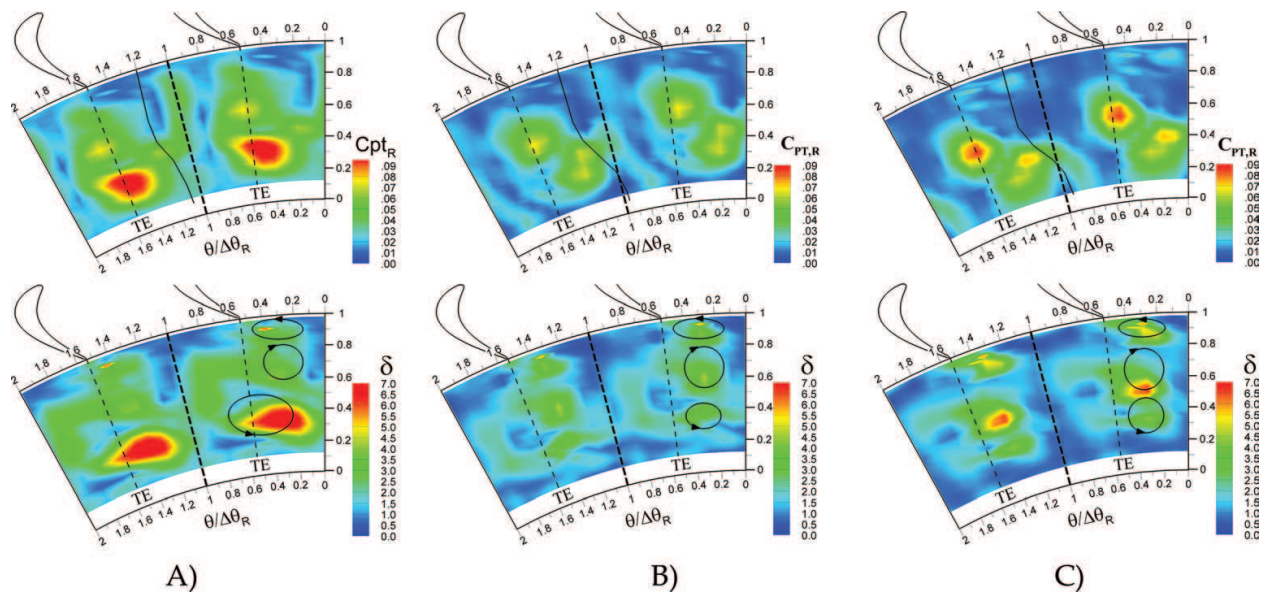
Figure 13. Standard deviation for the different instants of the interaction phases. (A) axial gap: x/bs = 16\% ; (B) axial gap: x/bs = 35\% , nominal; (C) axial gap = 50%. Experiments at the Fluidmachinery Lab. at Politecnico di Milano (Italy).
