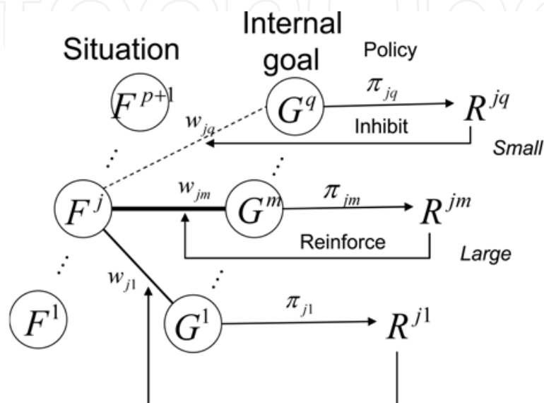
Fig. 6. Internal goal switching module
