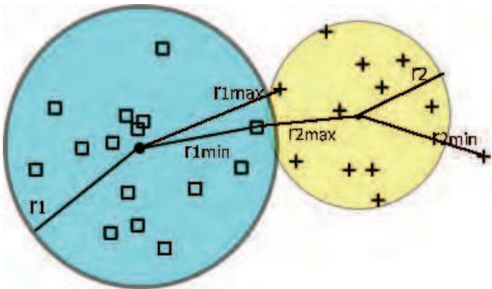
Fig. 11. Reduction of radios is applied to the left cluster and the right cluster is disregarded because it is not possible to do it.
