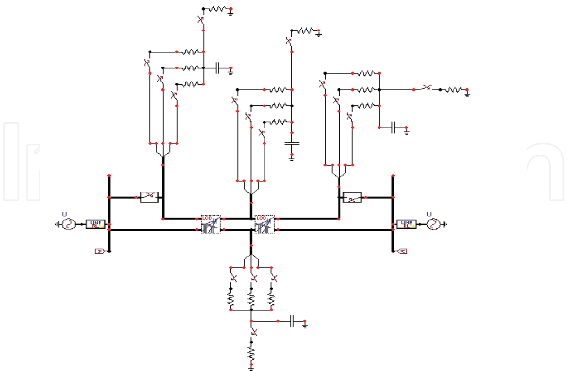
Fig. 16. Typical electrical circuit for analyzing conditions of faults in a SEP. (Alternative Transient Program-ATP).
