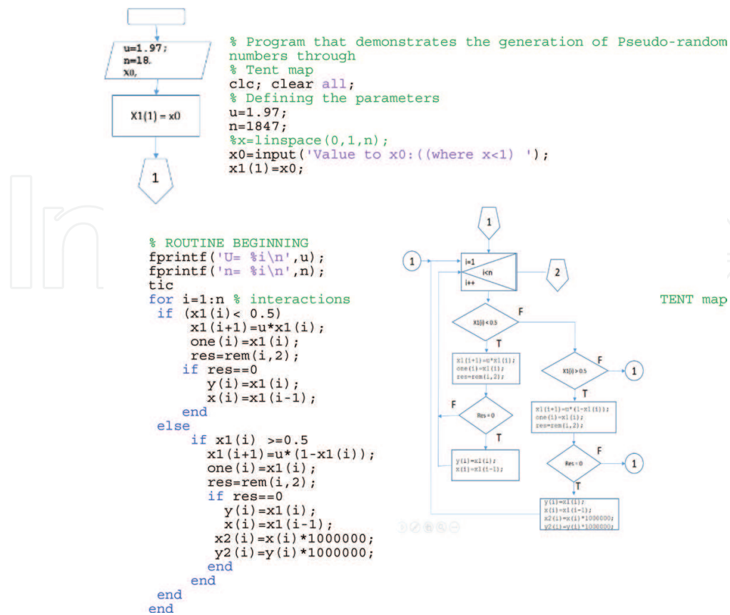
Figure 9. Algorithm by tent map.
