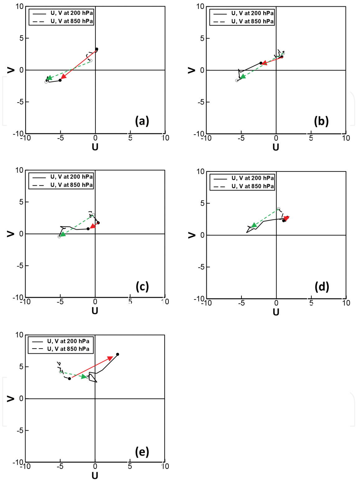
Figure 12. Changes in the averaged zonal wind (U, unit: \text{m s}^{-1} ) and meridional wind (V, unit: \text{m s}^{-1} ) within 500 km of the TC center for TCs making landfall in (a) Hainan, (b) Guangdong, (c) Taiwan, (d) Fujian, and (e) Zhejiang. The open and solid circles represent the 9 points (at every 6 h) starting at 24 h prior to landfall and ending at 24 h after landfall, respectively. The black solid lines are wind changes at 200 hPa, and the black long dashed lines are wind changes at 850 hPa. The green (red) dashed lines represent the vertical wind shear at 24 h prior to (24 h after) landfall.
