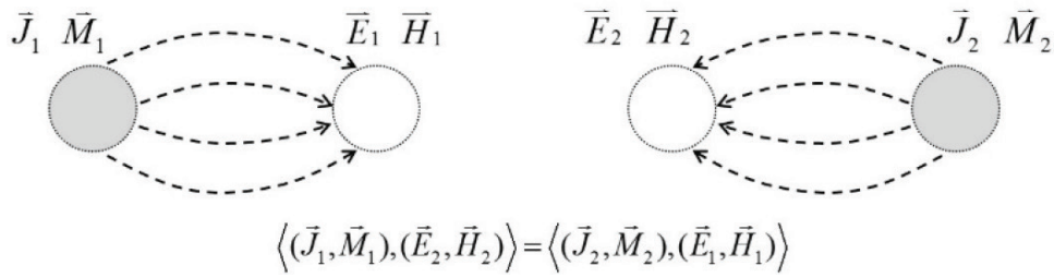
Figure 8. Reciprocity theorem.
