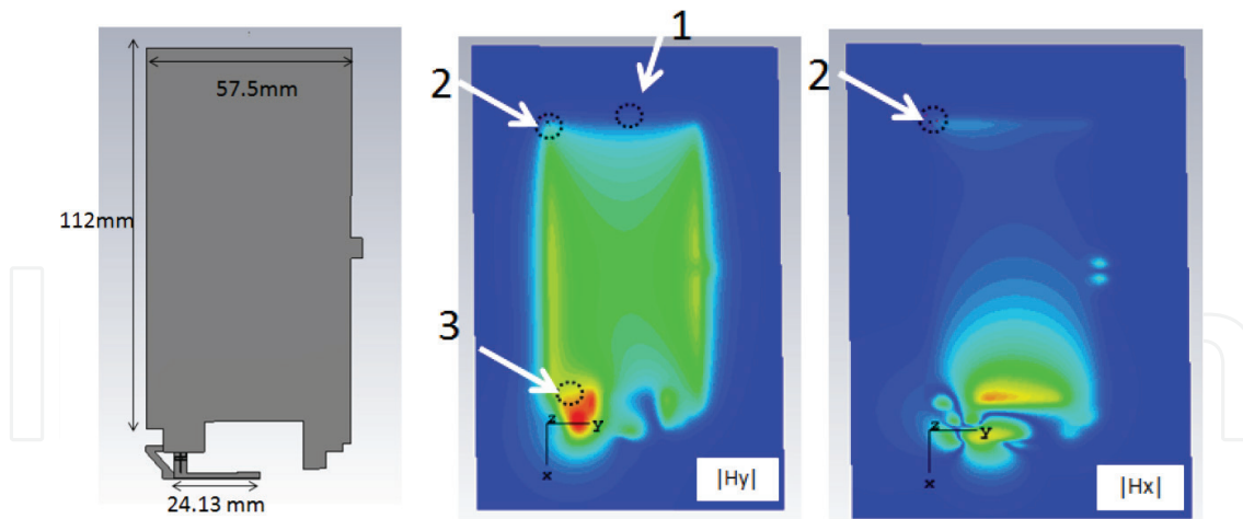
Figure 17. A typical cell phone antenna model (left), magnitude of H_y when the antenna radiates (center), and magnitude of H_x when the antenna radiates (right).
