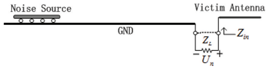
Figure 9. Original RF desensitization problem.
