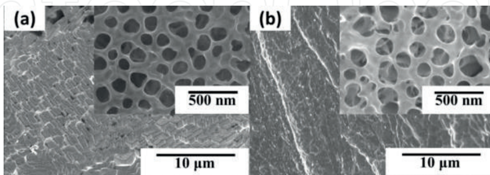
Figure 25. SEM image of foil's surface: (a) After 30 s etching (inset shows anodization after 1 h at 60 V) and (b) after 90 s etching [72].
