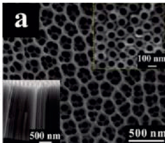
Figure 23. (a) SEM image of top view of porous \text{TiO}_2 nanotubes; Top enlarged image shows the diameter and bottom enlarged image shows the side walls [42].
