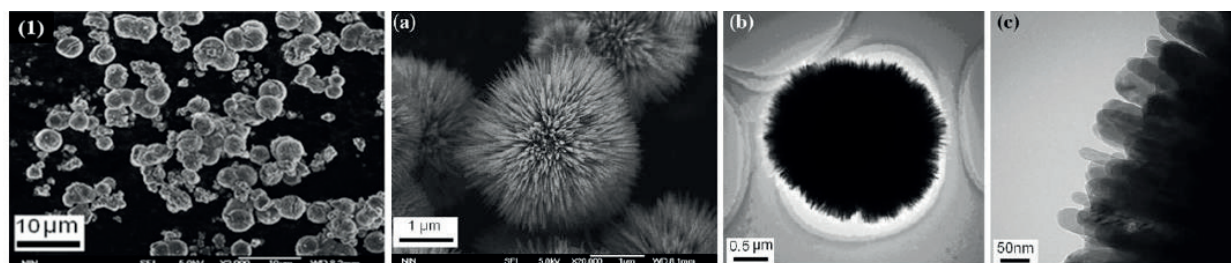
Figure 13. SEM images (1) nonhierarchical \text{TiO}_2 structures grown at 90^\circ\text{C} . (a–c) TEM images of 3D hierarchical urchin-like structures having 1D nanoneedles [35].
