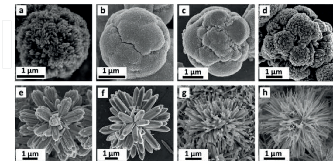
Figure 4. FESEM images of \text{TiO}_2 structures. Change in morphology is produced from changing HCl conc. at (a) 1M (b) 2M (c) 3M (d) 4M (e) 5M (f) 6M (g) 7M (h) 8M [56].
