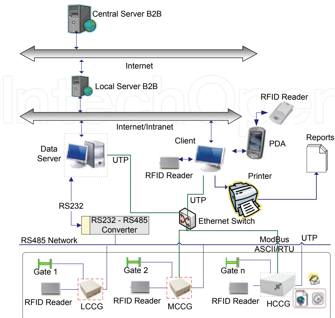
Fig. 1. The RFID_B2B system architecture
