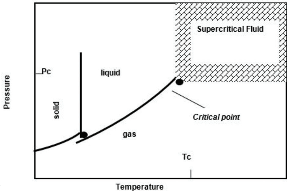
Figure 1. SCF temperature-pressure diagram.
