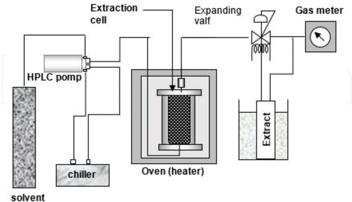
Figure 2. SFE system.
