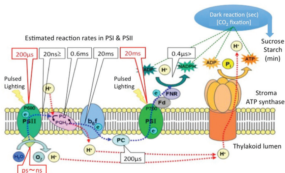
Figure 9. Photochemical reactions of photosynthesis are connected by an electron transport chain (ETC) between Photo-system I (PSI) and II (PSII), and ATP synthase embedded in thylakoid membrane in chloroplast. ETC composes of PSII reaction center (P680), plastquinone (PQ), cytochrome b 6 f complex ( b 6 f ), plastocyanin (PC), PSI reaction center (P700), ferredoxin (Fd), ferredoxin-NADP + reductase (FNR). Each estimated electron transfer rate is an example from Refs. [3, 4].
