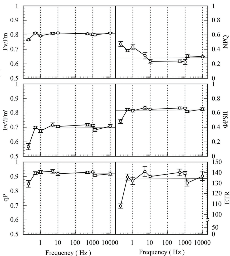
Figure 7. Chlorophyll fluorescent parameters of leaves grown under non-pulsed continuous lighting (horizontal line) and under different pulsed lighting cycles (○). F_v/F_m and F_v'/F_m' were measured with dark-adapted or exposing leaves to 500 \mu\text{mol m}^{-2} \text{s}^{-1} PPFD (saturated irradiance with or without pulse cycles) to estimate photochemical ( qP ) and non-photochemical ( NPQ ) quenching.
