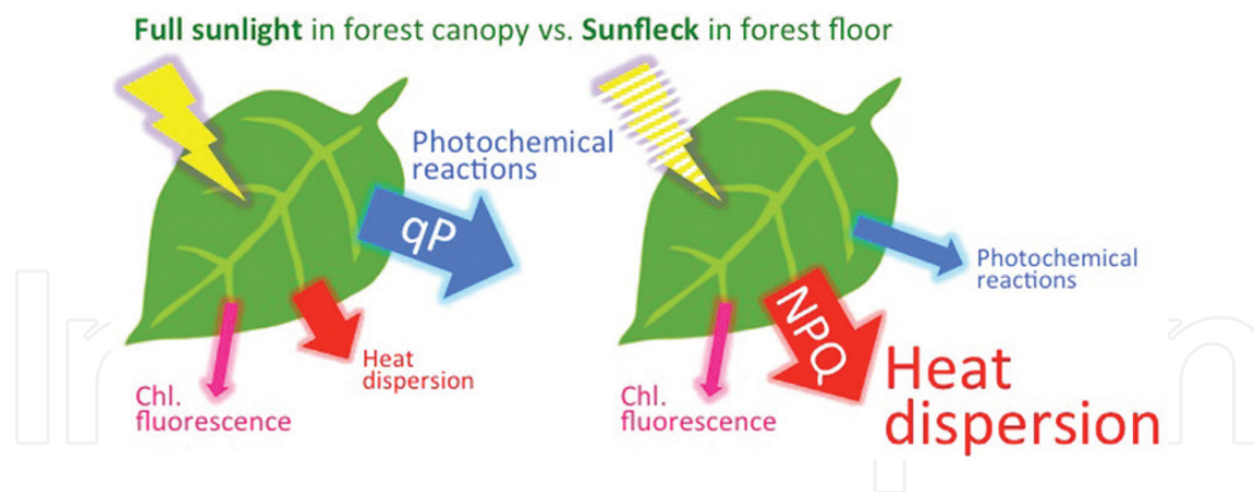
Figure 8. Photochemical reactions of photosynthesis of leaf lettuce are affected by exposing leaves to slow flash pulsed strong lighting (<1 Hz). An instantaneous response of PS by enhancing heat dissipation from leaves exposed to natural sunfleck in forest floor where plants are protected against photoinhibition.
