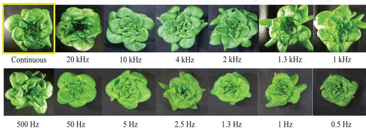
Figure 4. Leaf lettuce hydroponically grown under different pulsed lighting for 20 days.
