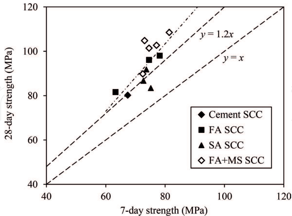
Figure 3. Plot of 28-day strength versus 7-day strength.
