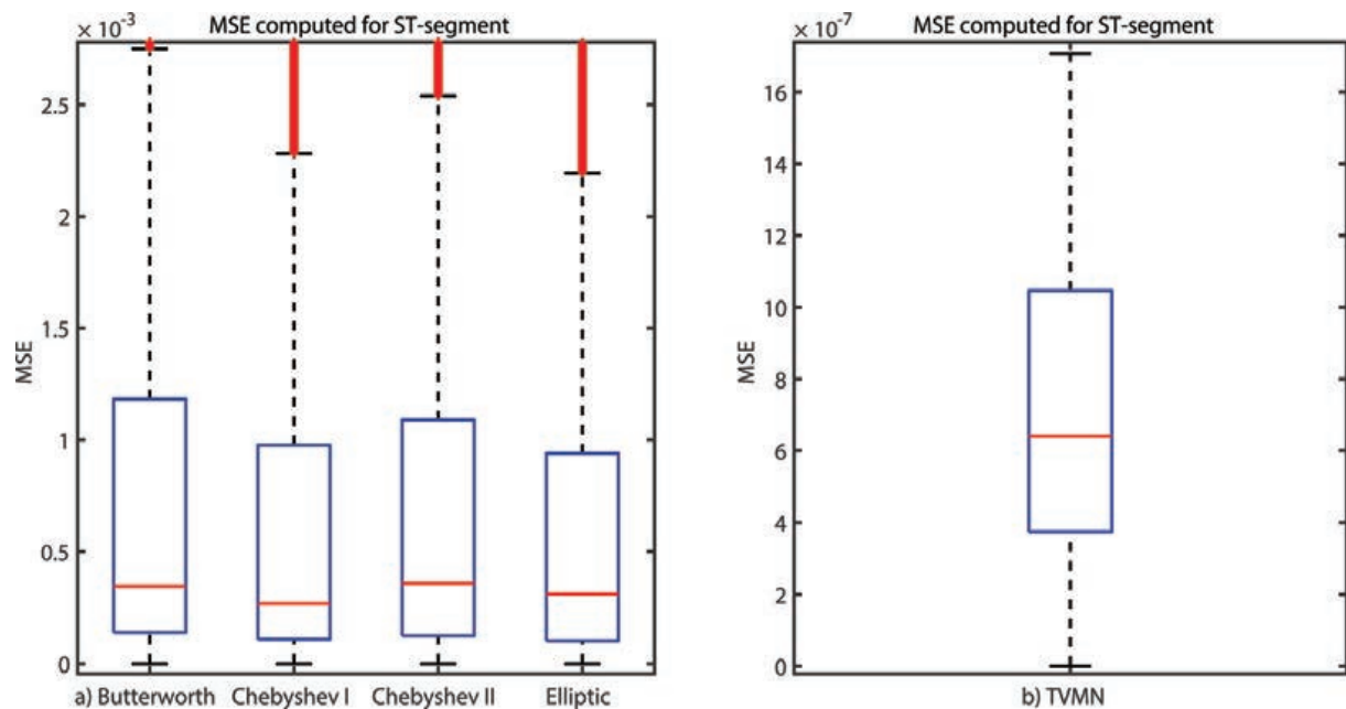
Figure 11. MSE determined for all 19,715 ST segments: (a) after the digital traditional band stop filters are applied; (b) after the TVMN is applied.
