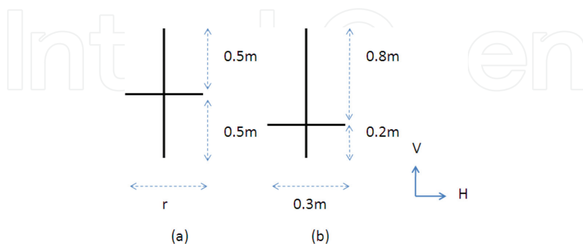
Figure 5. Wire targets and corresponding excitation polarization references. (a) Target 1: r = 0.3\text{ m} , target 2: r = 0.2\text{ m} , and (b) target 3 (reprinted from [47] with permission from IEEE).
