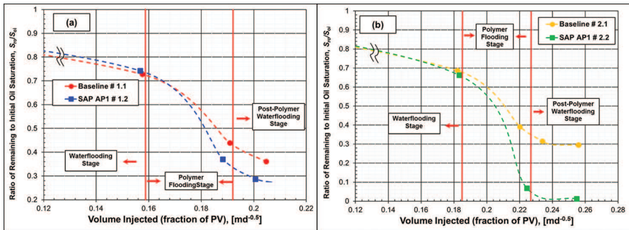
Figure 5. S_{ro}/S_{oi} versus volume of fluid injected and flooding stage: (a) Baseline # 1.1 and SAP-AP1 # 1.2 and (b) Baseline # 2.1 and SAP-AP1 # 2.2.
