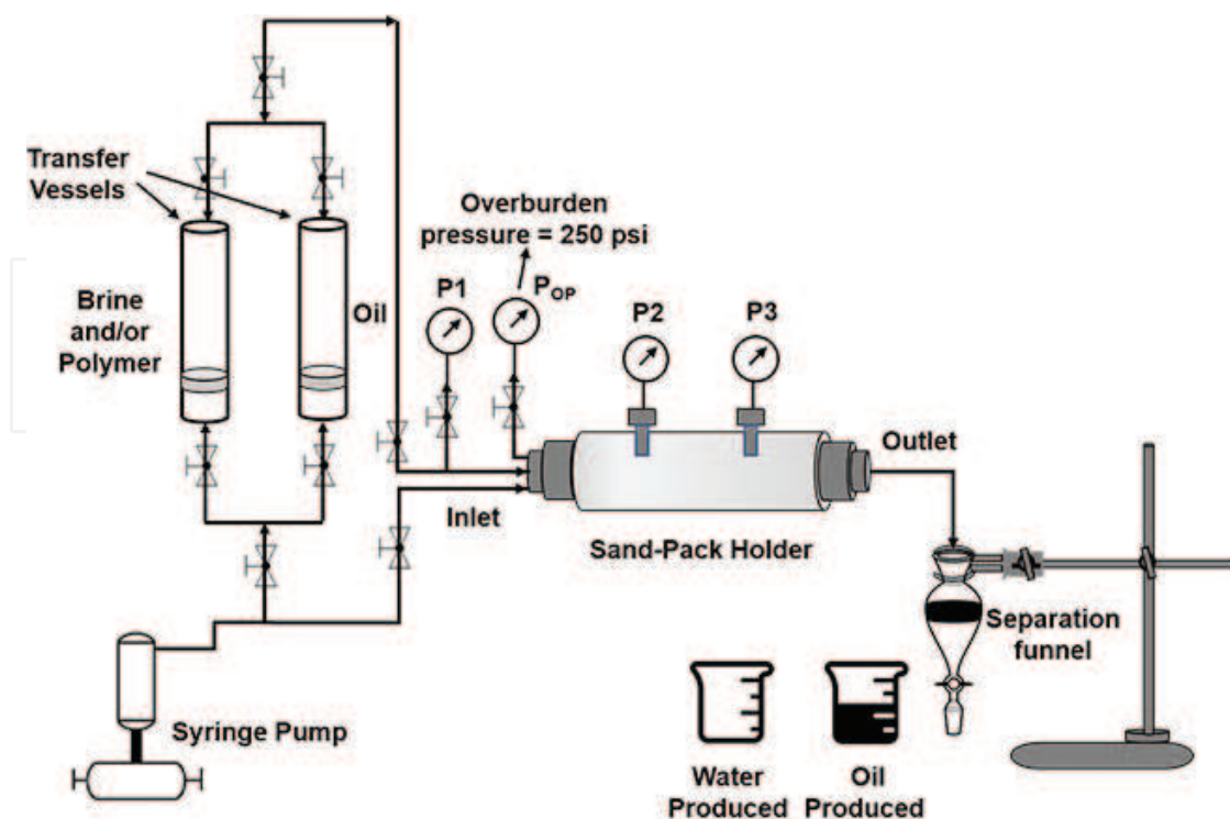
Figure 1. Experimental set-up for sand-pack displacement tests.
