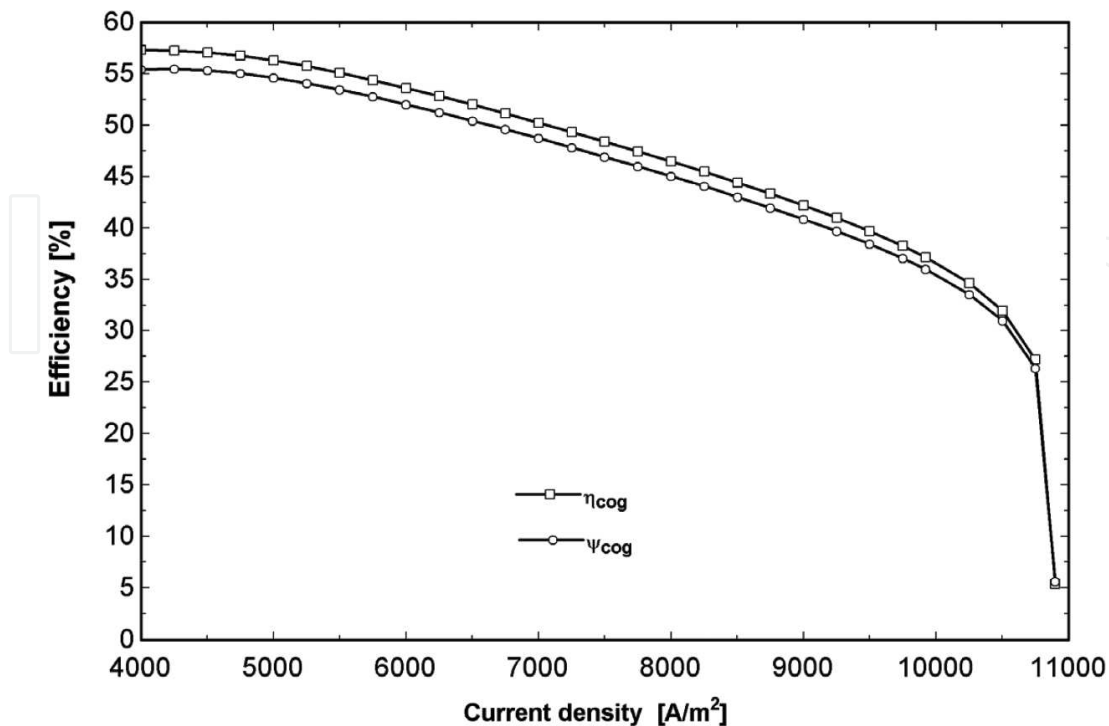
Figure 5. Variation of the cogeneration energy and exergy efficiencies with respect to current density.
