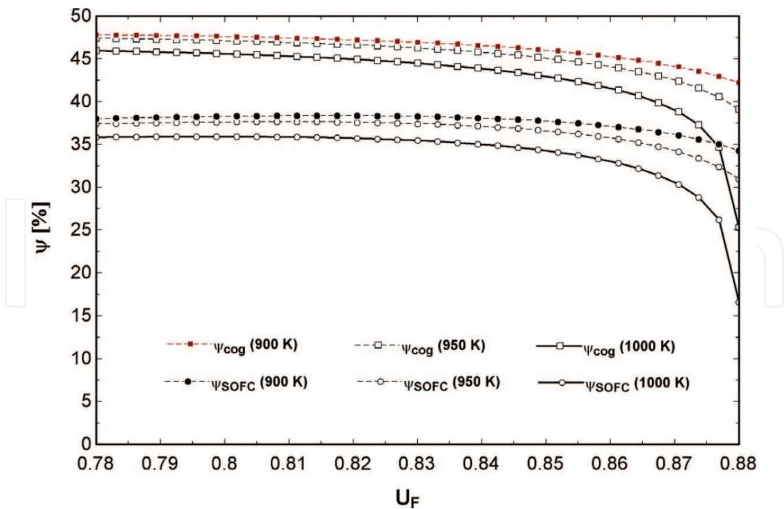
Figure 6. Variation of exergy efficiency with U_F at three different inlet fuel temperatures.
