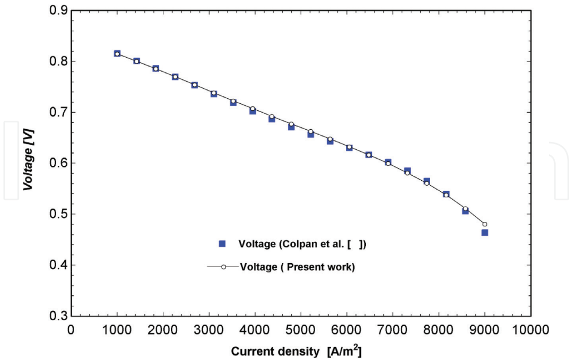
Figure 2. Characteristic polarization curve.
