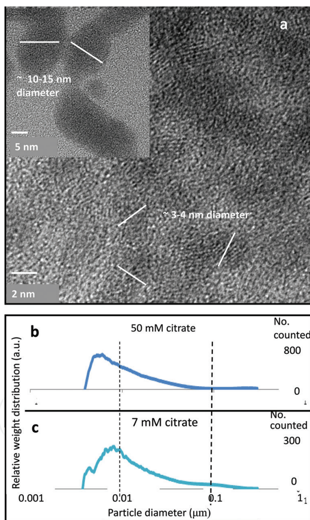
Figure 11. High resolution TEM study and population size analysis of ZnS QDs made under two citrate concentrations. Biogenic \text{H}_2\text{S} was used to make ZnS in 50 mM citrate buffer (a, main image) and 7 mM citrate buffer (a, inset). Approximate respective nanoparticle sizes are 3–4 and ~10 nm as shown. The population from 7 mM citrate solution had additional small nanoparticles of size ~5 nm (a, inset). Bars are 2 and 5 nm as shown. b,c: Estimation of nanoparticle sizes using an analytical disc centrifuge as described in [60] using light scattering. The nanoparticle size in 50 mM citrate buffer was calculated (from log plots) as ~4–5 nm and in 7 mM citrate buffer was ~8–10 nm with a smaller population of size <5 nm. The small nanoparticles are too close to the lower size cutoff of the instrument [60] to be an exact measurement, but the two independent methods report the same result. Figure 11a was in collaboration with J. Gomez-Bolivar.
