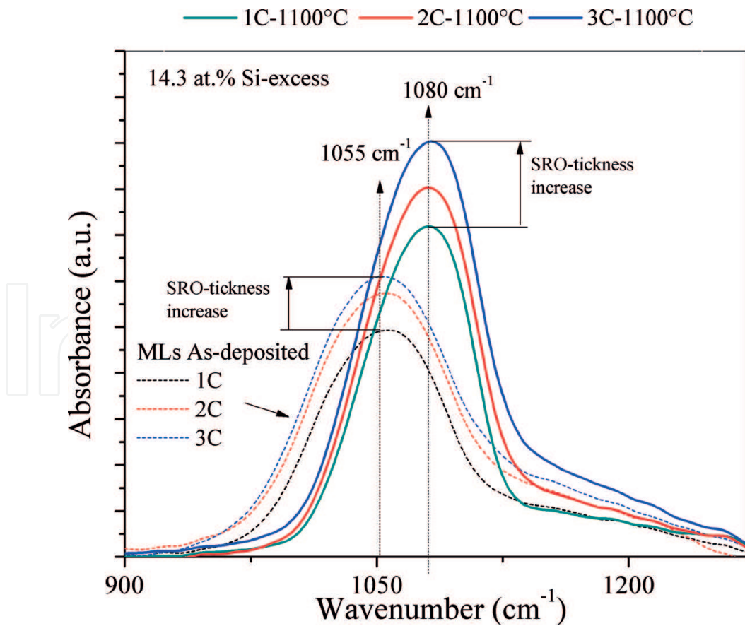
Figure 7. FTIR spectra of SRO/SiO 2 MLs as function of SRO-thickness (2.5–7.5 nm) of as-deposited and thermally annealed at 1100°C.
