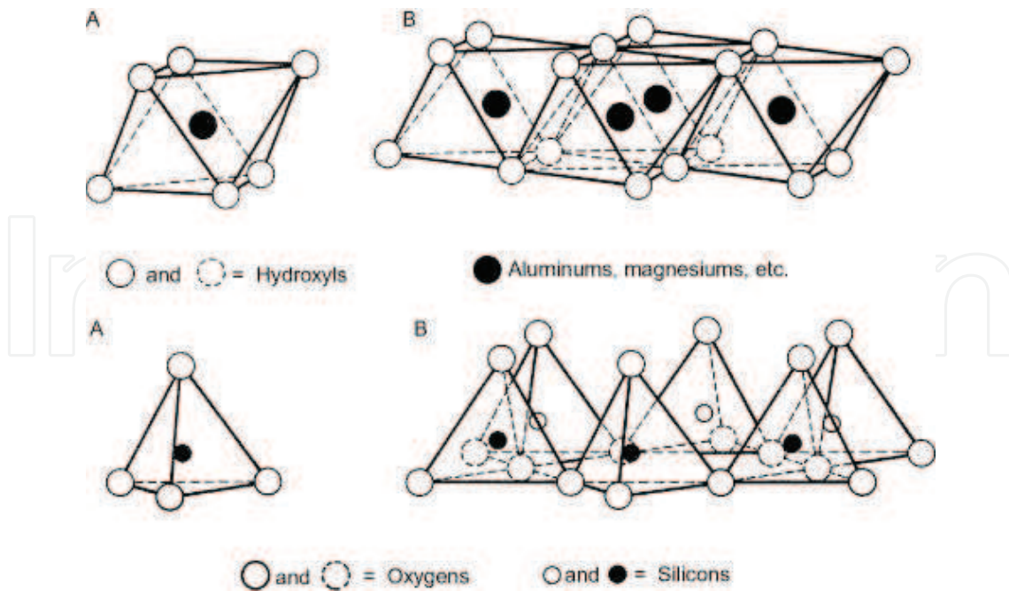
Figure 1. Schematic diagrams of octahedron and tetrahedron sheets. Top: (A) an alumina octahedron in which the central aluminum ion is coordinated to six hydroxyls; (B) an alumina octahedral sheet formed by linking octahedra through edge-sharing. Bottom: (A) a silica tetrahedron in which the central silicon ion is coordinated to four oxygens; (B) a tetrahedral sheet formed by linking silica tetrahedra through corner-sharing [11].
