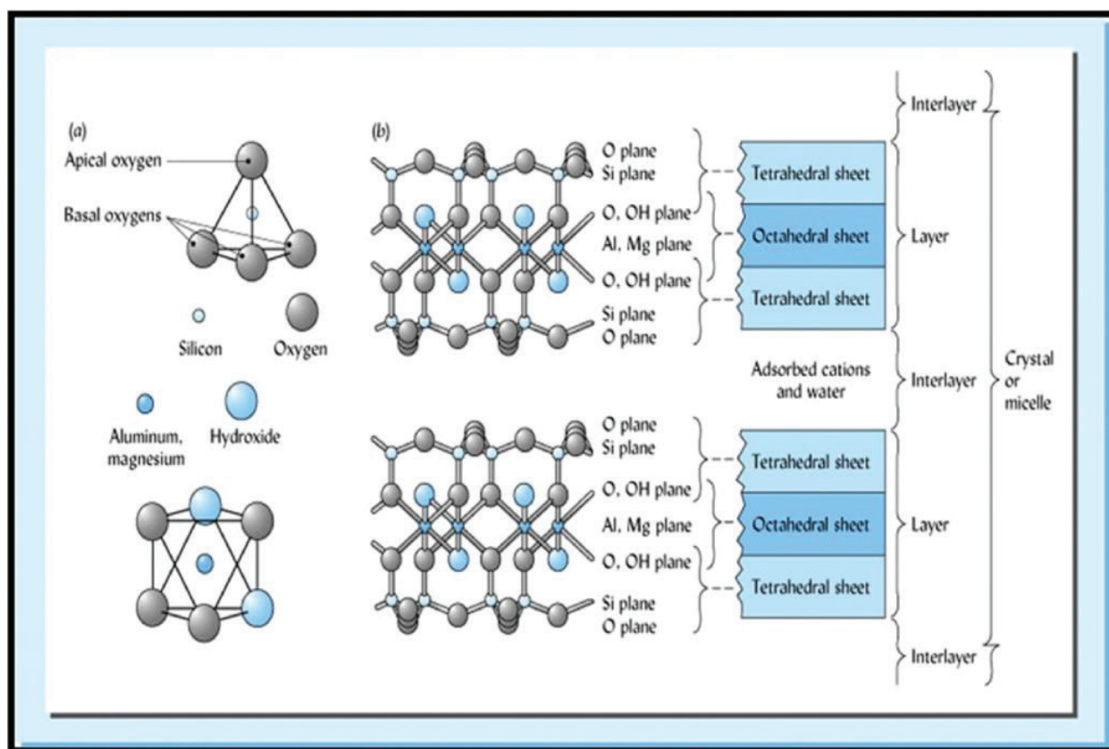
Figure 3. Typical structure of 2:1 clay [19].
