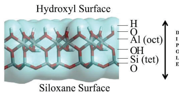
Figure 2. Typical structure of Kaoline mineral [15].
