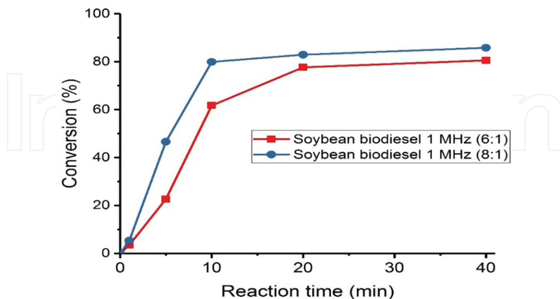
Figure 11. Soybean biodiesel by ultrasound using the 1 MHz transducer using an alcohol/oil ratio of 6:1 and 8:1.
