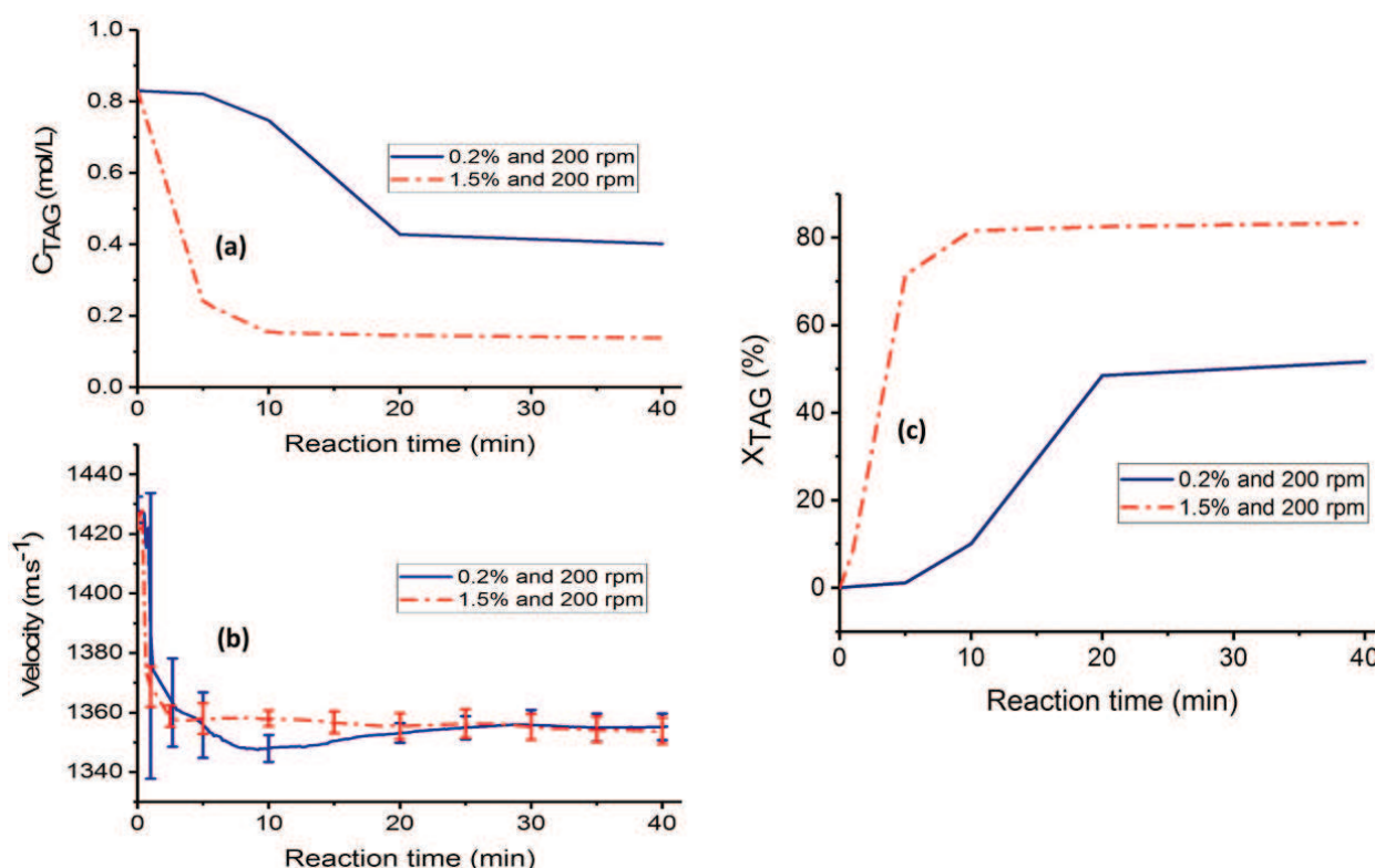
Figure 12. Variation of (a) TAG concentration, (b) propagation velocity and (c) TAG conversion for the reactions with 200 rpm of rotation. Reprinted from Baêso et al. [9].
