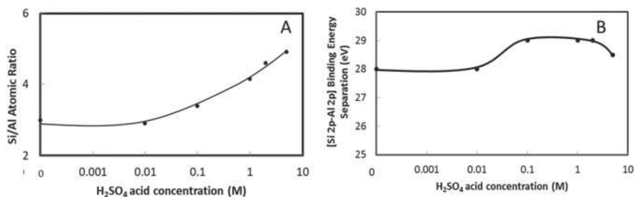
Figure 8. The effect of increasing acid concentration on Si/Al ratio (A) and [\text{Si}_{2p}-\text{Al}_{2p}] binding energy separations (B) (trend line included to illustrate the relationship) [29].
