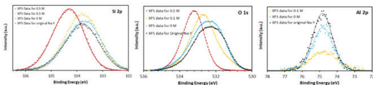
Figure 13. XPS high-resolution spectra of original and sulfuric acid-treated Na–Y for \text{Si}_{2p} , \text{O}_{1s} , and \text{Al}_{2p} [34].
