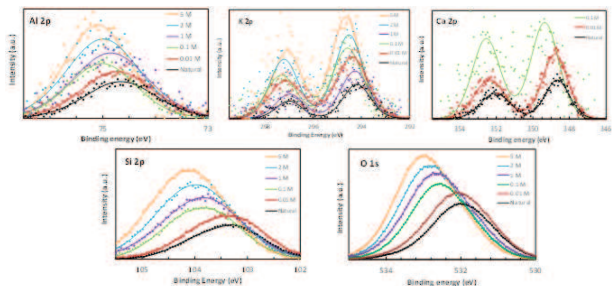
Figure 9. XPS high-resolution spectra of natural and acid-modified zeolite for \text{Si}_{2p} , \text{Al}_{2p} , \text{O}_{1s} , \text{K}_{2p} , and \text{Ca}_{2p} [29].
