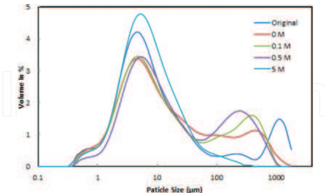
Figure 14. Particle size distribution of original and acid-treated Na–Y [34].
