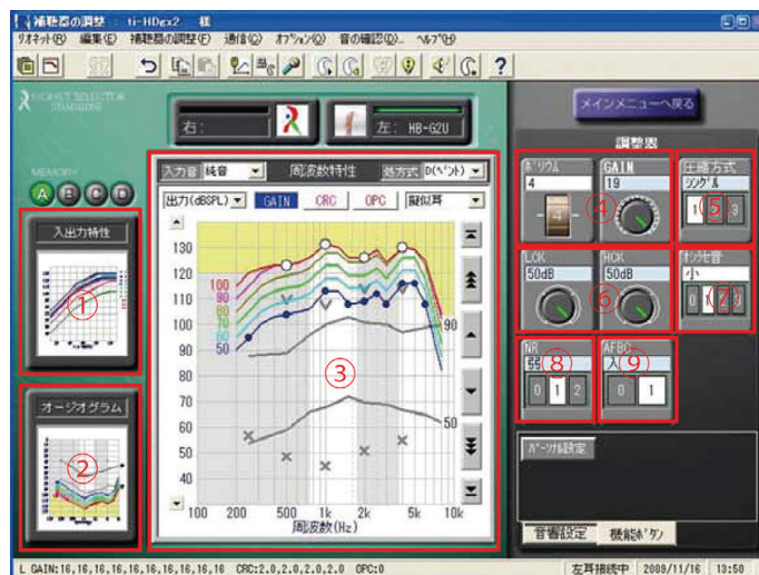
Figure 6. Example of software used to adjust a hearing aid's digital signal processing.
