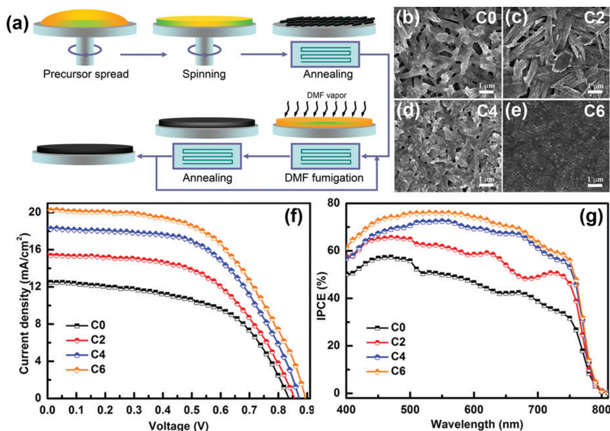
Figure 6. (a) Schematic processing procedure for MAPbI 3 film deposition (C0) and recrystallization via DMF vapor fumigation for 2 (C2), 4 (C4), and 6 (C6) cycles. (b–e) Surfacial SEM images of samples C0, C2, C4, and C6. (f) J–V curves and (g) IPCE spectra of the devices based on samples of C0, C2, C4, and C6, respectively. Reproduced with permission from Ref. [45]. Copyright 2015, Royal Society of Chemistry.
