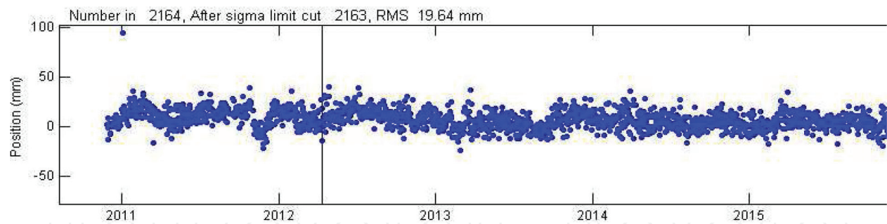
Figure 5. Example of stability of reference station from repeatability of their height component position through years of observation.
