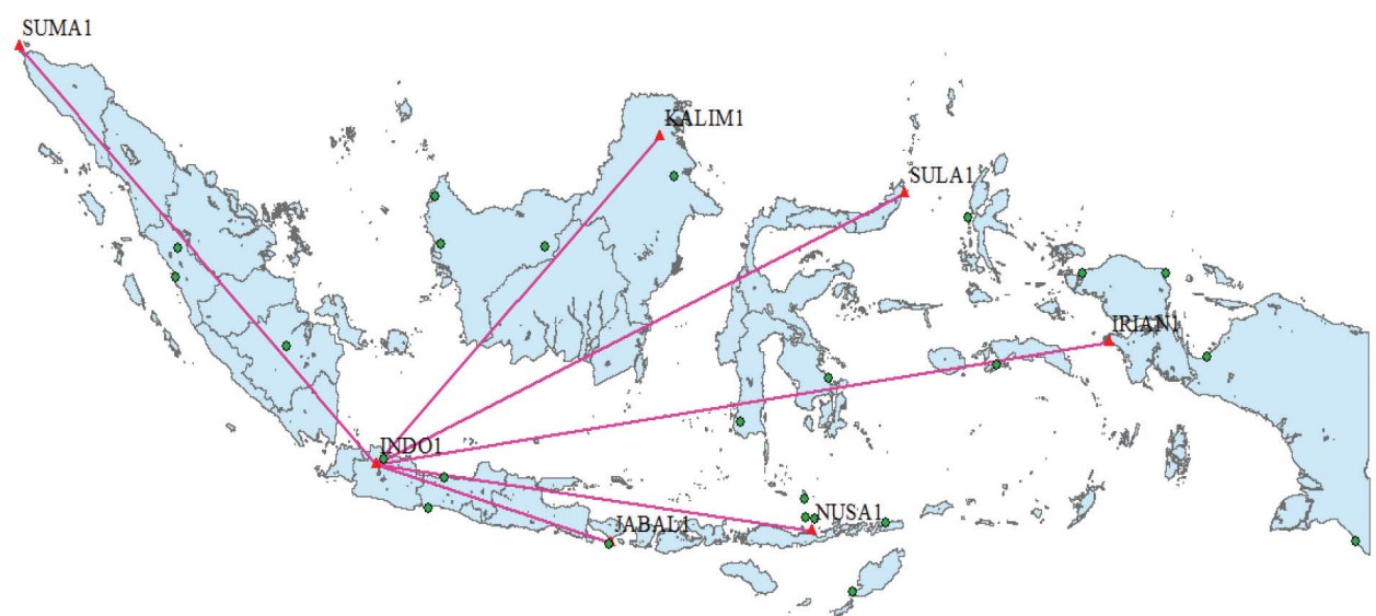
Figure 8. Baseline concepts using one stable reference station for subsidence monitoring along large offshore oil and gas area of Indonesia.
