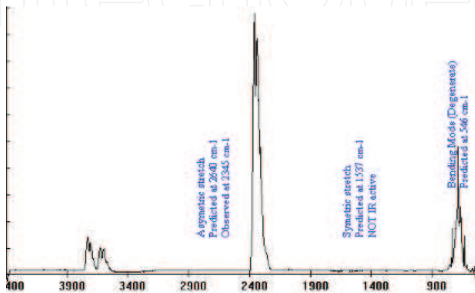
Figure 6. IR spectra of CO 2 . The fundamental vibrations of molecules belonging to the D ∞h point group are similar in type to those of the nonsymmetrical linear molecules, but in this instance, they may also be symmetric (v s ) or antisymmetric (v as ) to the center of symmetry, and thus σ g , σ u , π g , and π u modes, two stretching and two bending (degenerate) vibrations. The v as (CO) mode and the degenerate δ(OCO) mode involve changes in the dipole moment during the vibration, and they are IR active. Thus, v as has been observed by IR as a very strong parallel-type band at 2349.3 cm -1 , while δ(OCO) appears as a strong perpendicular-type band at 667.3 cm -1 .
