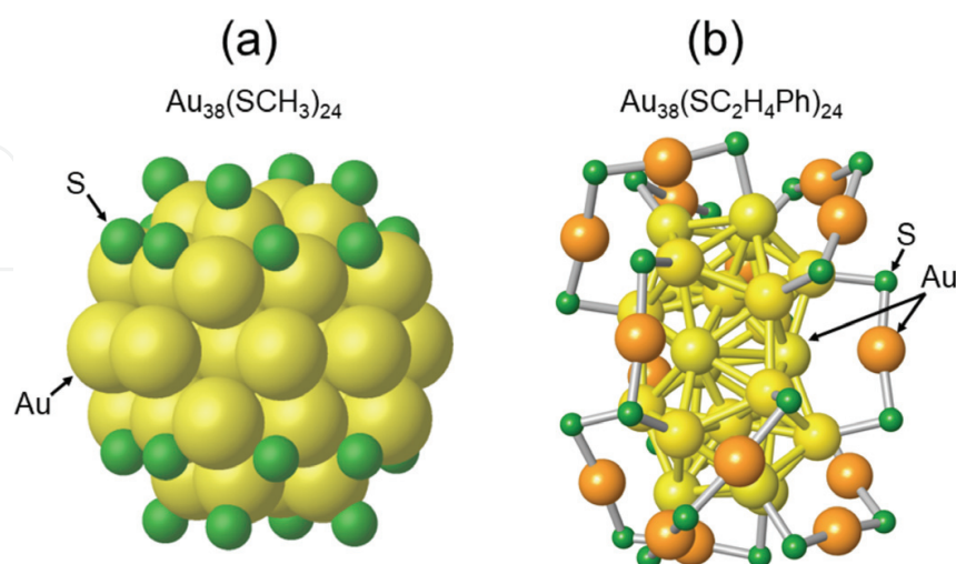
Figure 3. The geometrical structures of \text{Au}_{38}(\text{SR})_{24} (a) predicted by theoretical calculations in 1999 and (b) determined by single-crystal X-ray structural analysis in 2010. The R groups have been omitted for clarity (these figures were adapted from Refs. [30, 84]).
