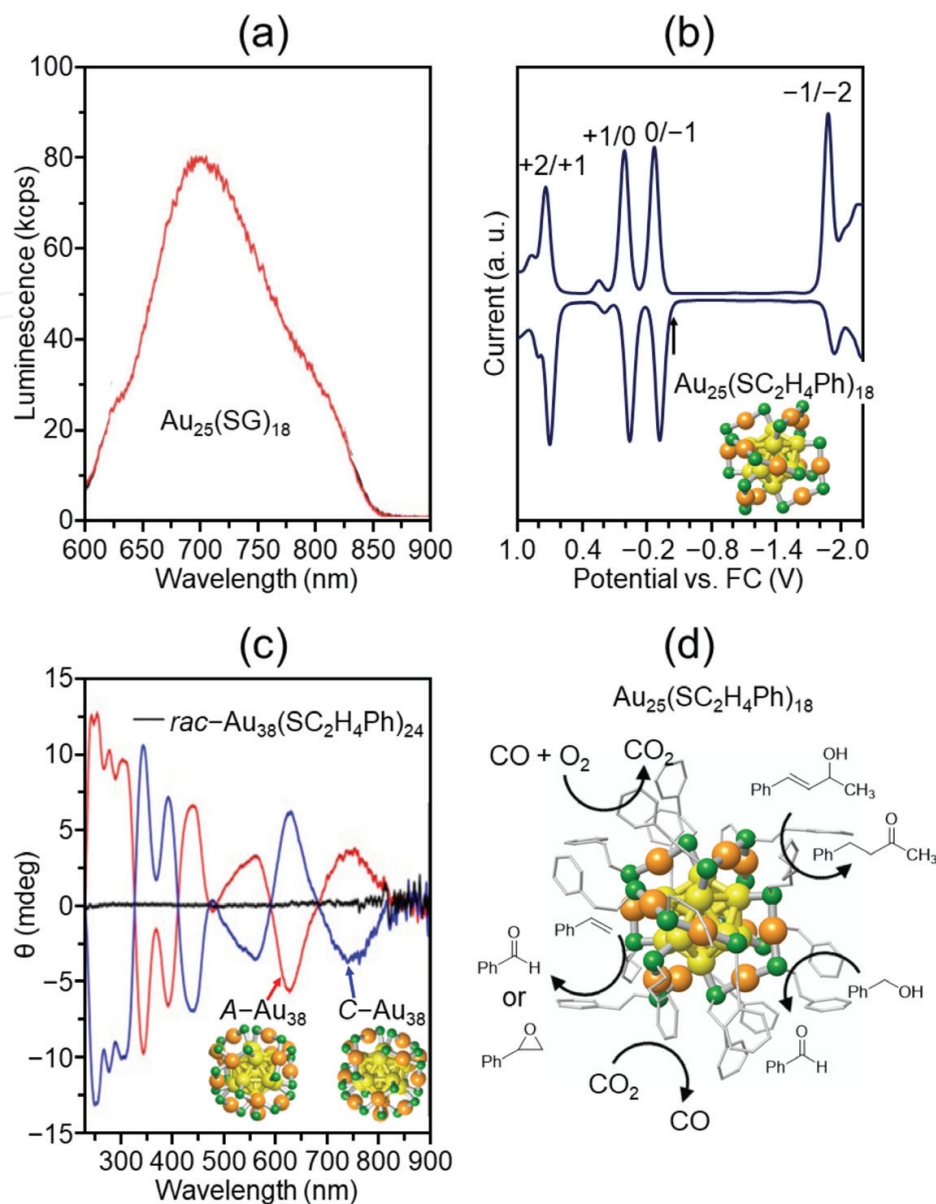
Figure 6. Size-specific physical and chemical properties of \text{Au}_n(\text{SR})_m clusters: (a) photoluminescence, (b) redox behavior, (c) optical activity, and (d) catalytic activity (these figures were adapted from Refs. [22, 90, 95]).
