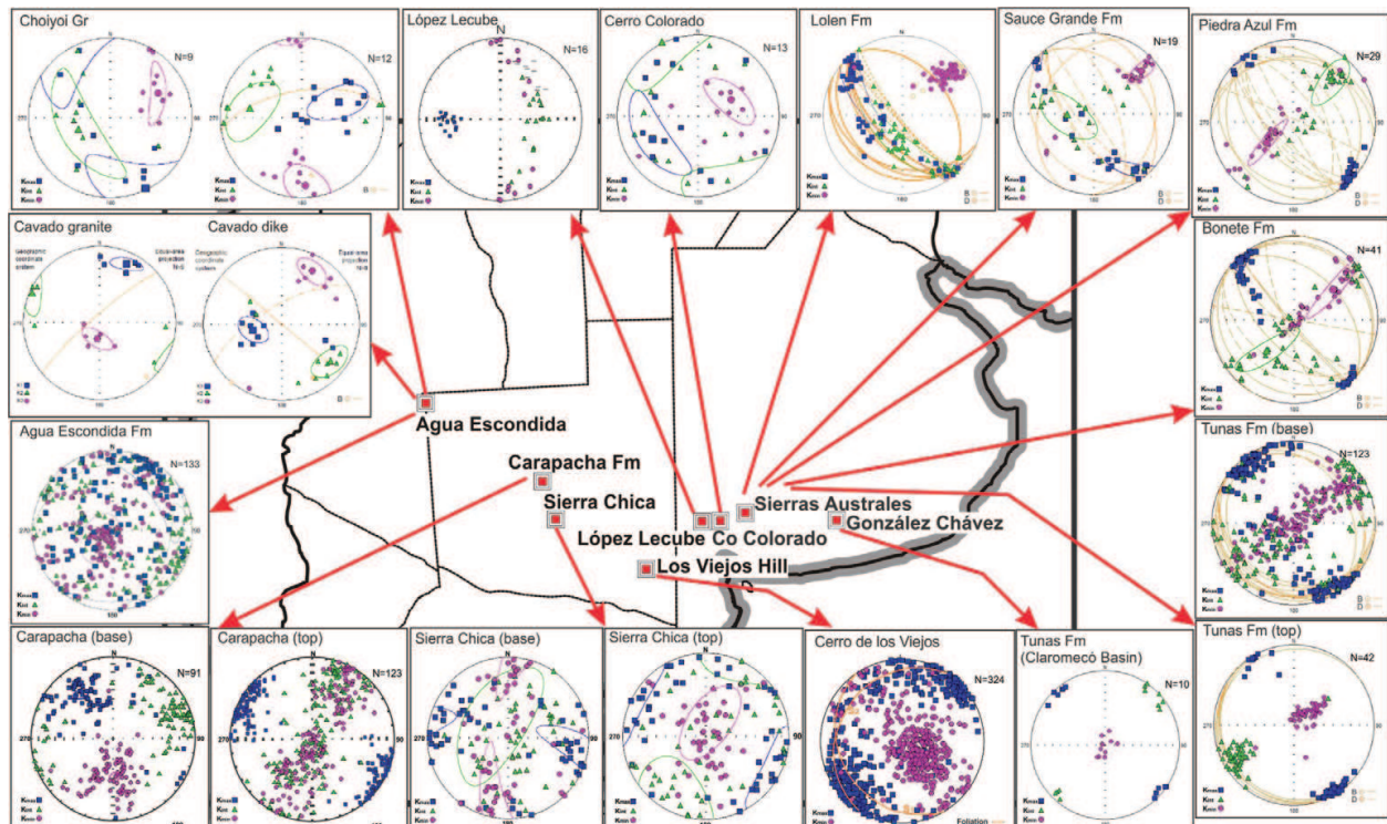
Figure 4. AMS ellipsoids results of the different sectors of the southwest margin of Gondwana, with the K_{\max} , K_{\min} and K_{\text{int}} axes and N the number of specimens. The stereographic nets are in geographic coordinate system and equal-area projection.
